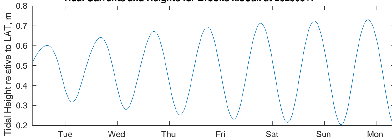
Tidal Currents and Heights for Brooks McCall at 20250317
