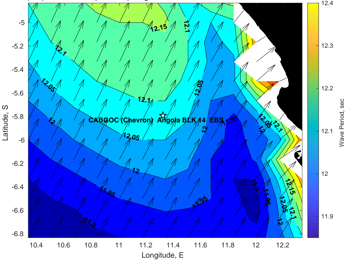
Wave Period (sec) for CABGOC (Chevron) Angola BLK 14 EBS at 14-Mar-2025 09:00:00
