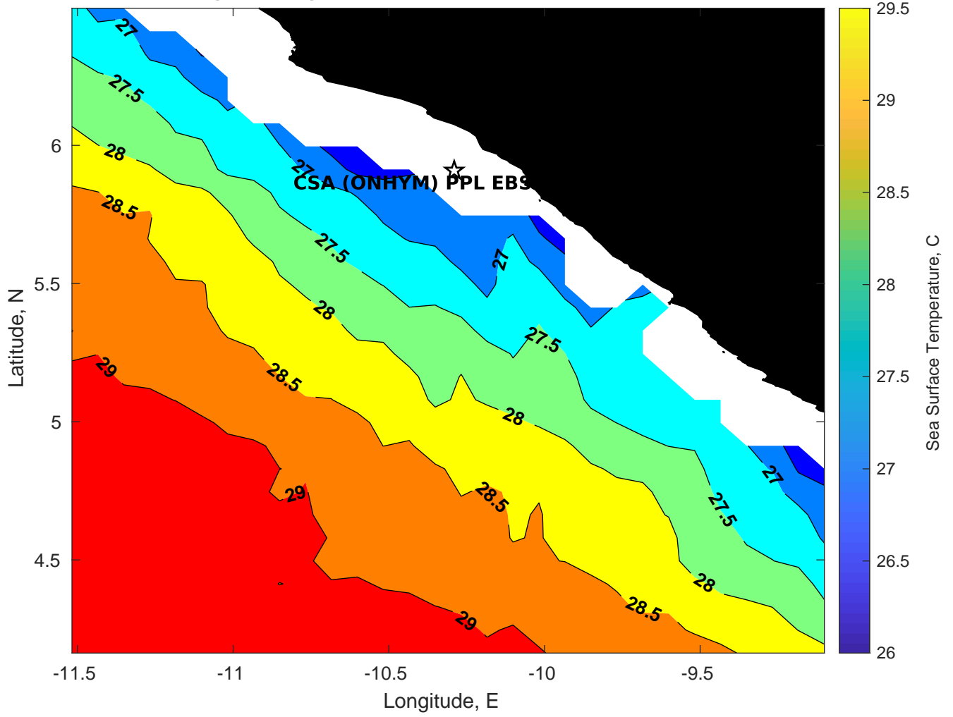
SST for CSA (ONHYM) PPL EBS - Liberia at 13-Mar-2025 00:00:00
