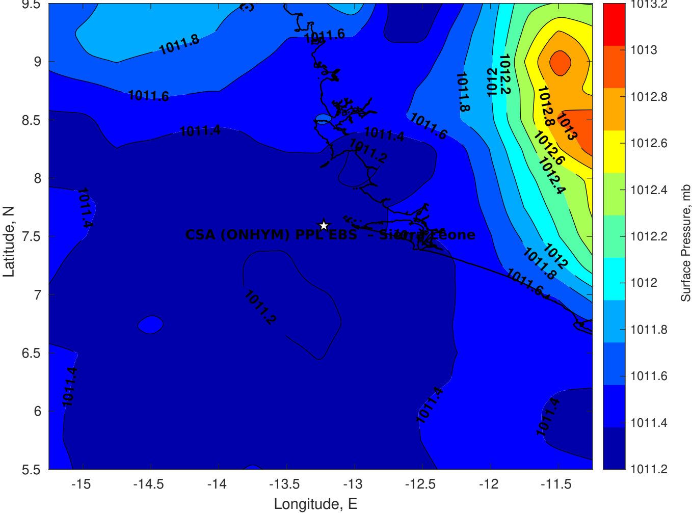
Surface Pressure (mb) for CSA (ONHYM) PPL EBS - Sierra Leone at 15-Mar-2025 00:00:00
