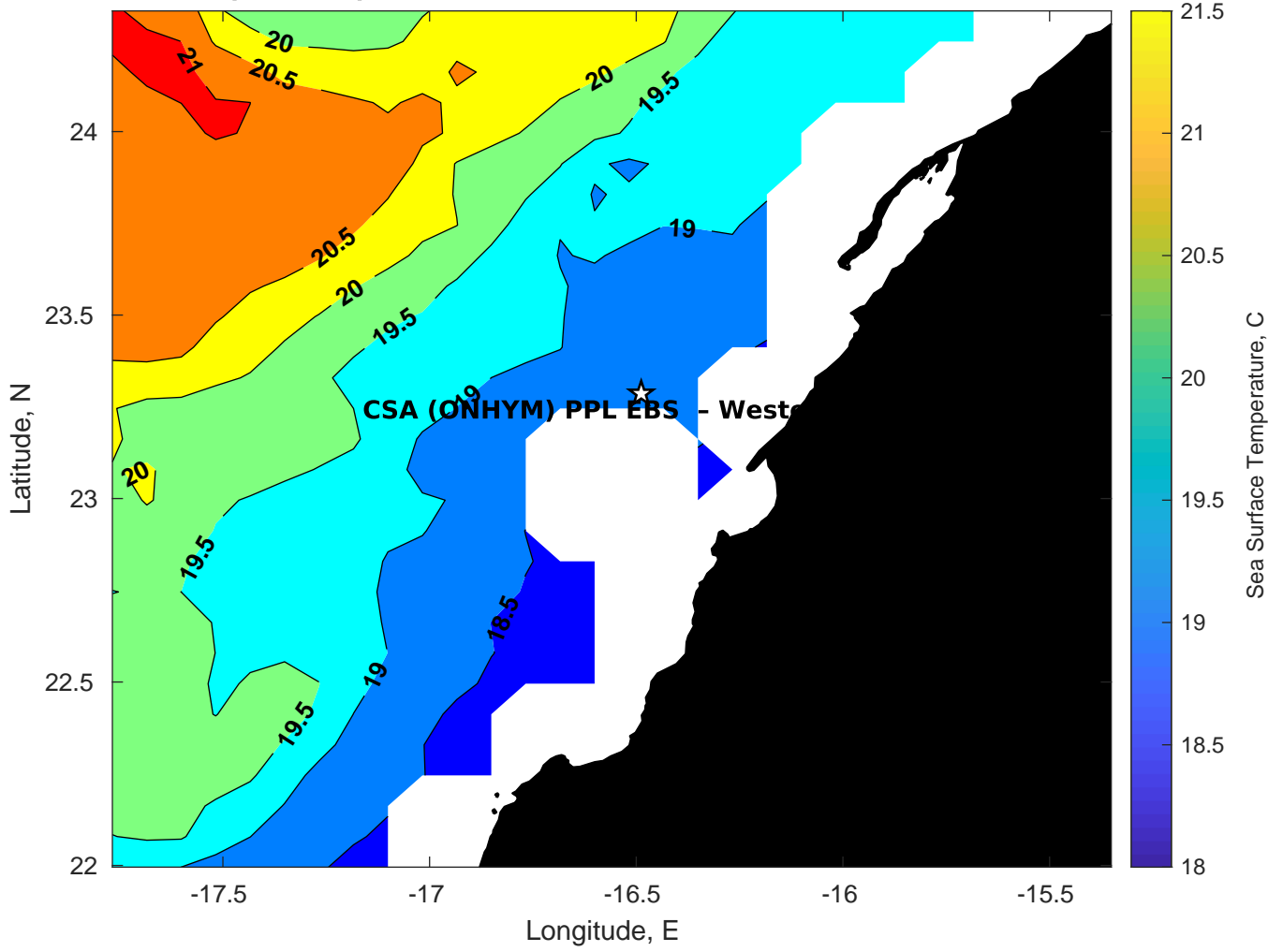
SST for CSA (ONHYM) PPL EBS - Western Sahara at 13-Mar-2025 00:00:00
