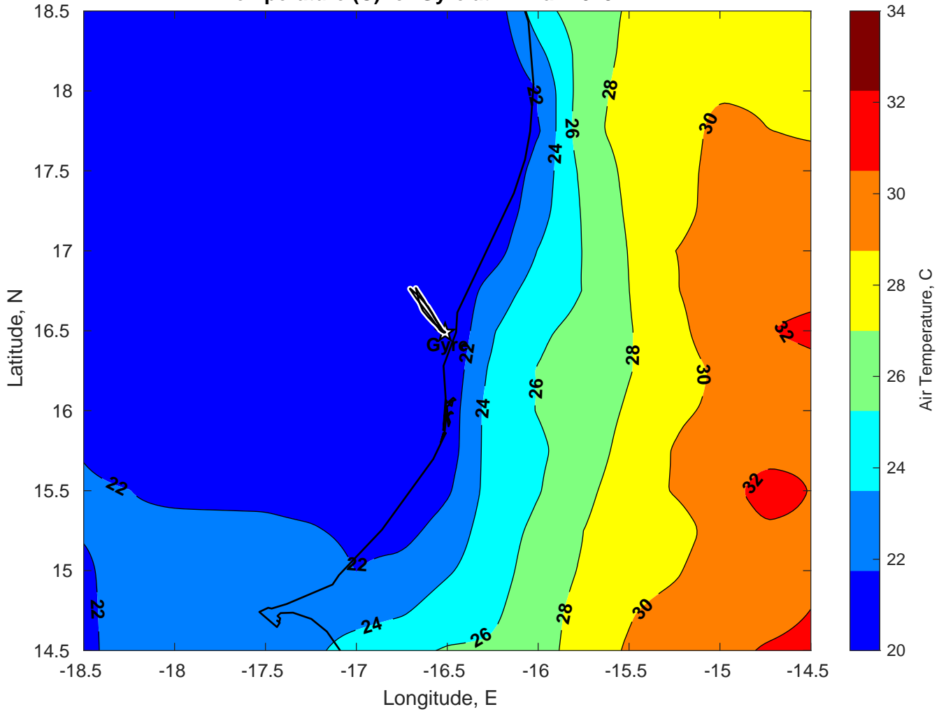
Air Temperature (C) for Gyre at 17-Mar-2025
