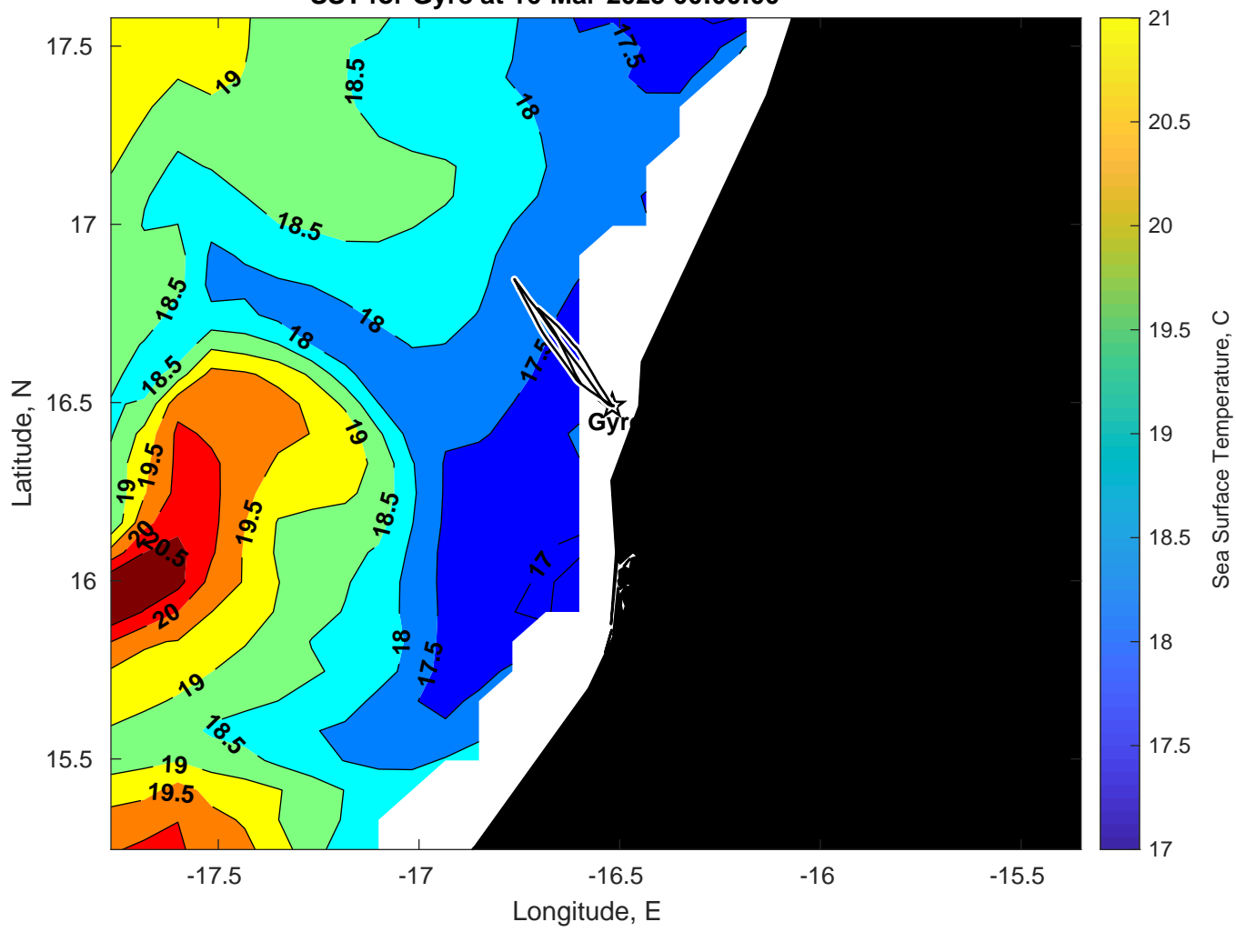
SST for Gyre at 16-Mar-2025 00:00:00
