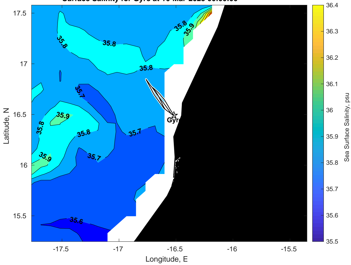
Surface Salinity for Gyre at 16-Mar-2025 00:00:00
