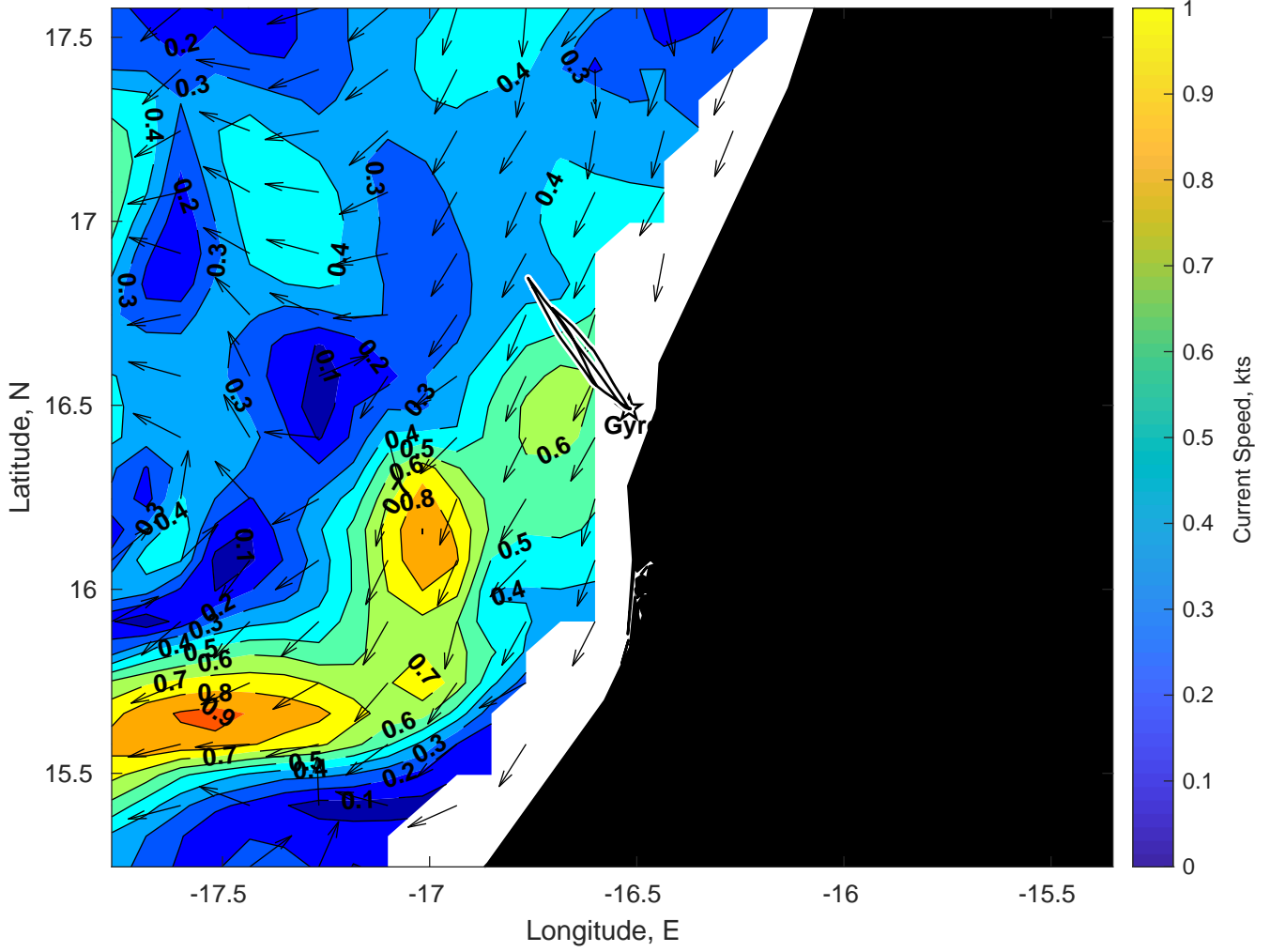
Surface Currents for Gyre at 16-Mar-2025 00:00:00
