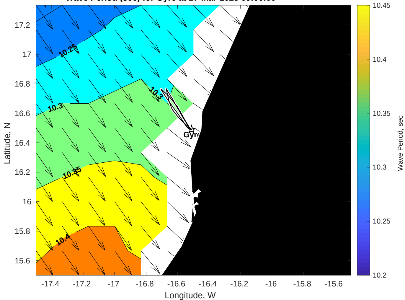
Wave Period (sec) for Gyre at 17-Mar-2025 09:00:00
