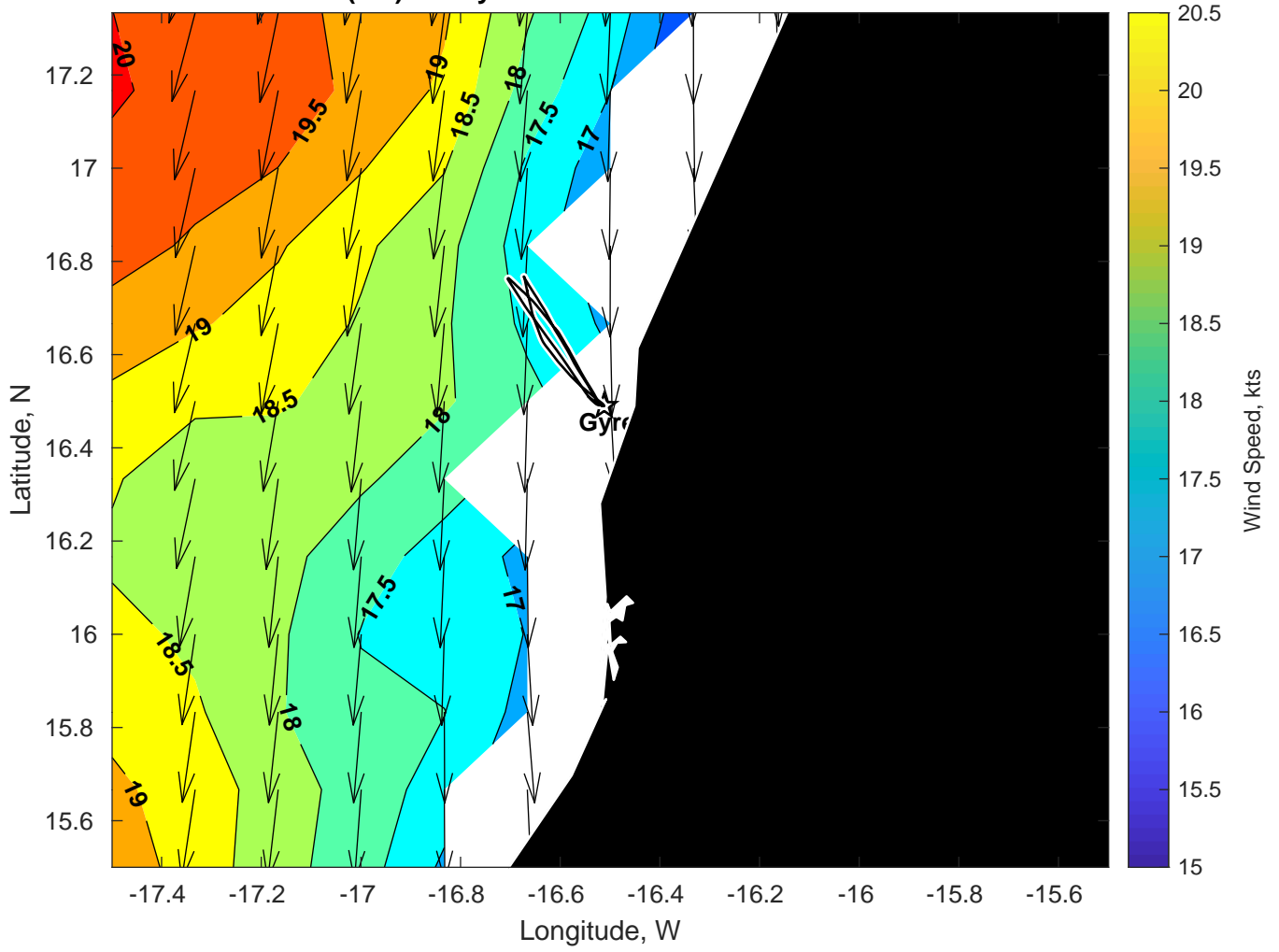
Winds (kts) for Gyre at 17-Mar-2025 09:00:00
