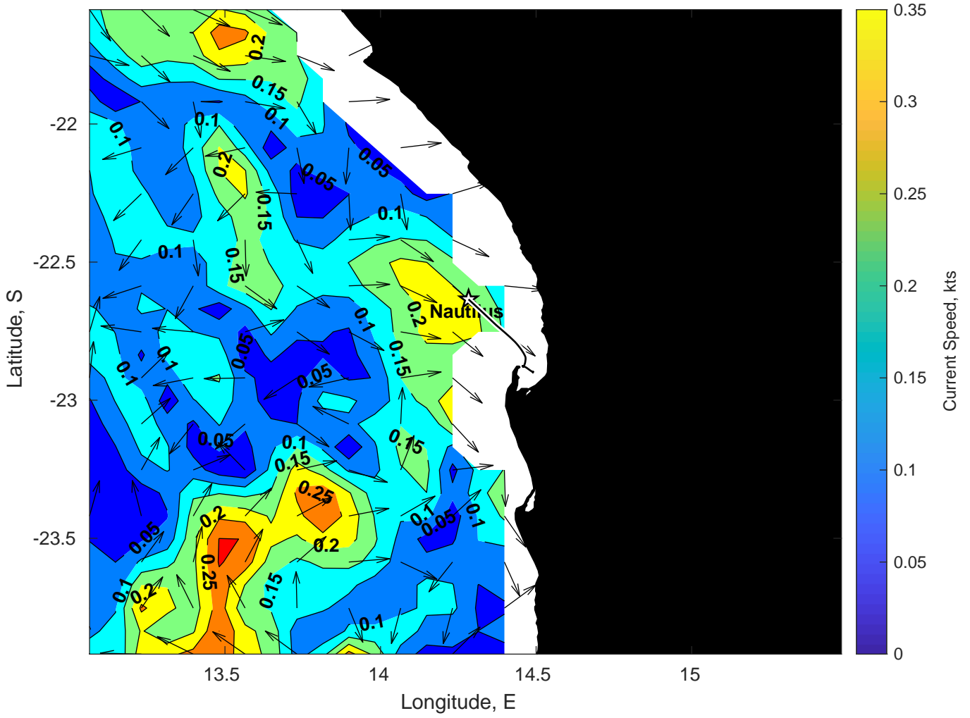
Surface Currents for Nautilus at 13-Mar-2025 00:00:00
