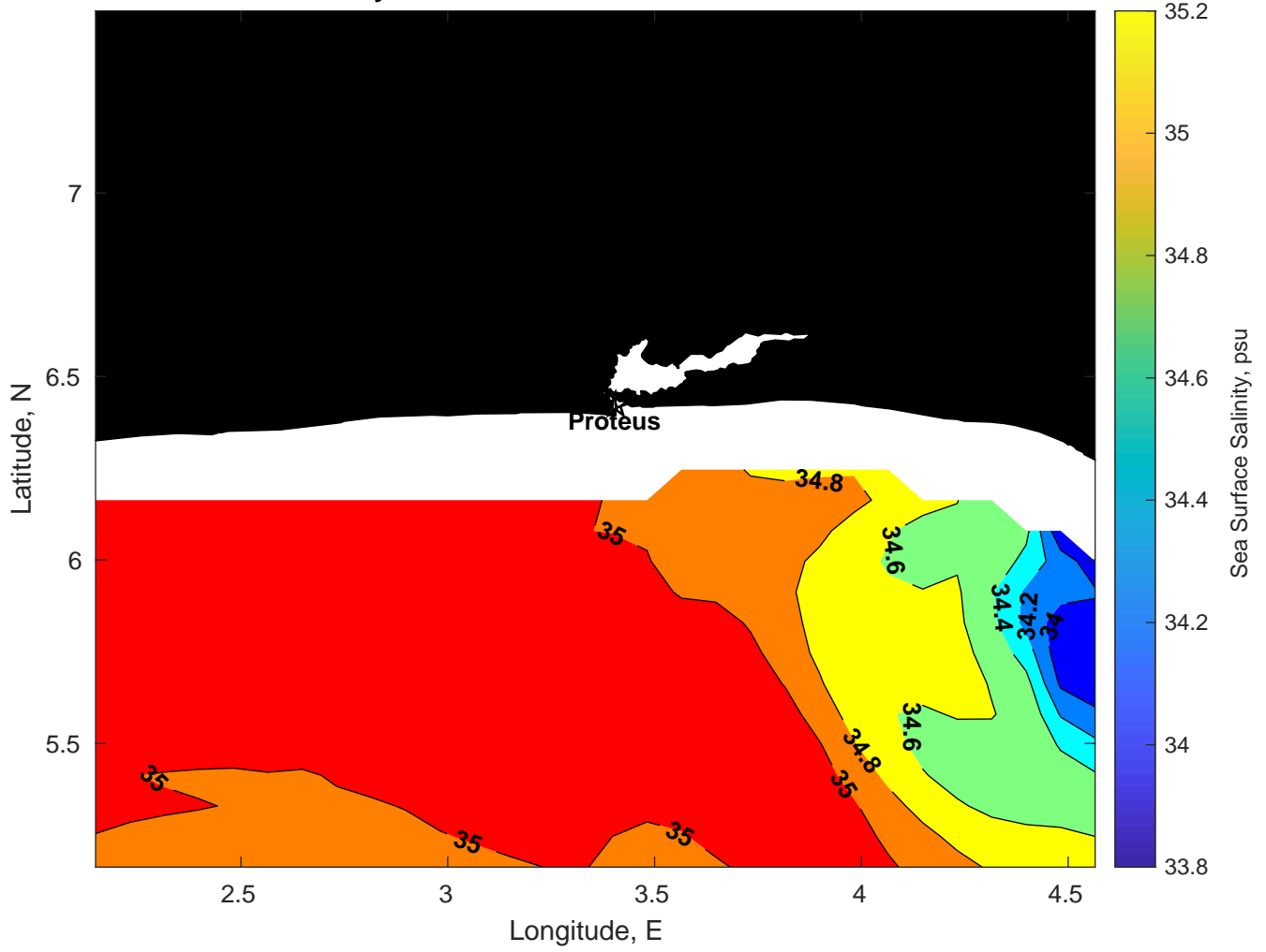
Surface Salinity for Proteus at 13-Mar-2025 00:00:00
