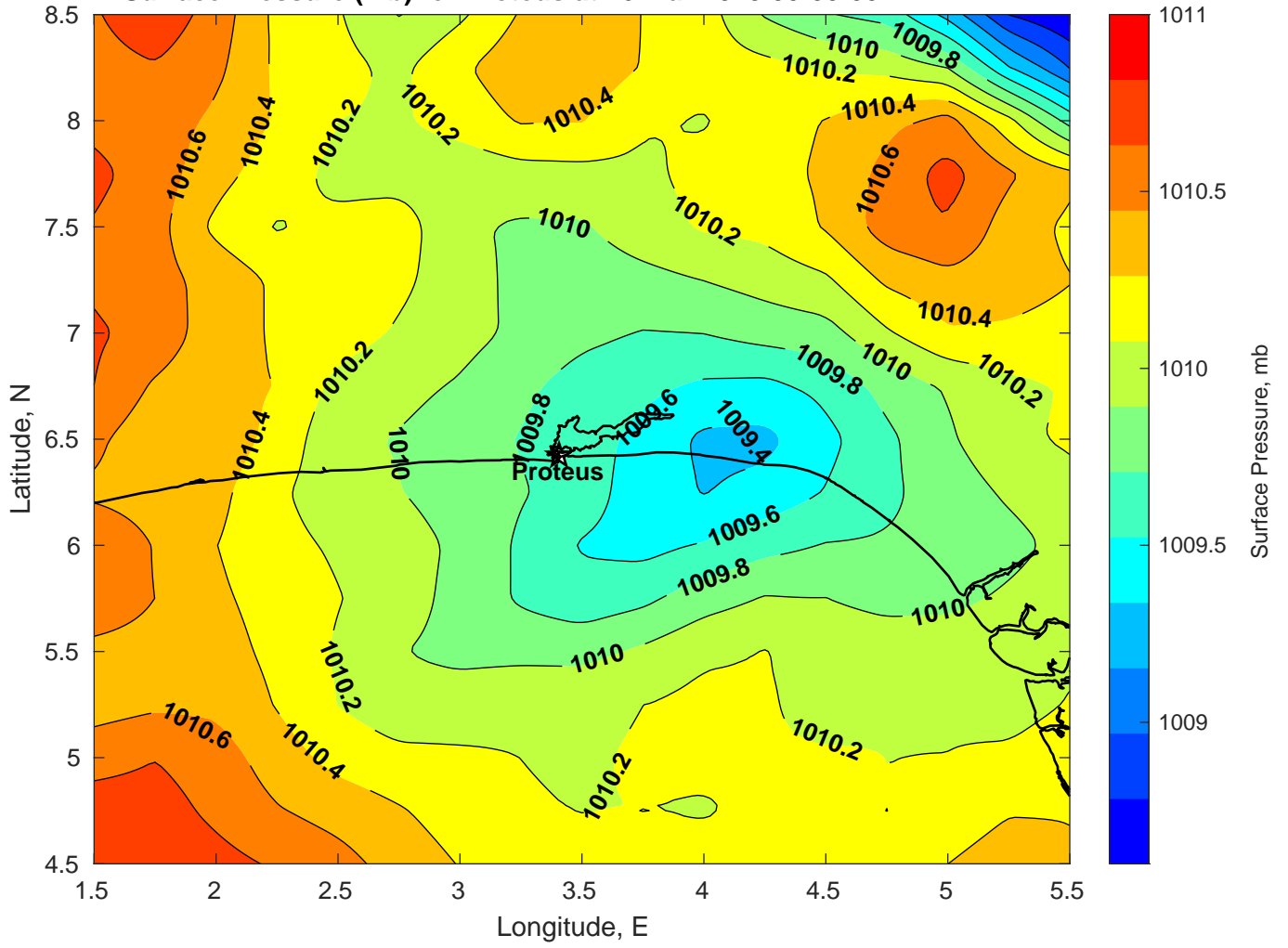
Surface Pressure (mb) for Proteus at 16-Mar-2025 00:00:00
