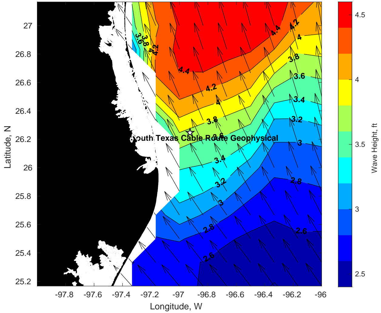
Wave Height (ft) for Tampnet P2378 South Texas Cable Route Geophysical at 14-Mar-2025 09:00:00
