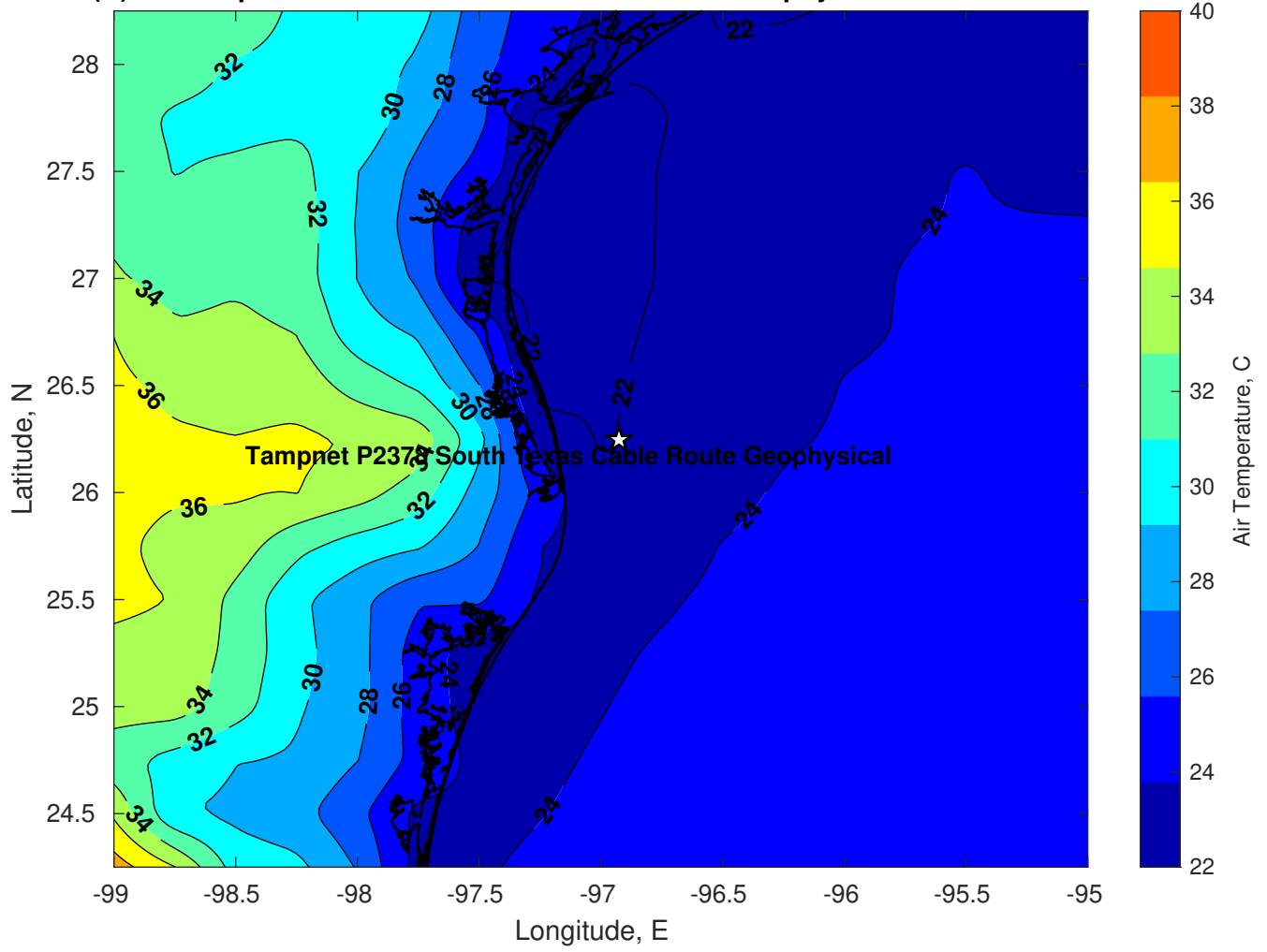
Air Temperature (C) for Tampnet P2378 South Texas Cable Route Geophysical at 14-Mar-2025
