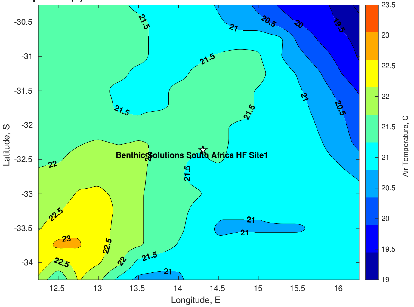
Air Temperature (C) for Benthic Solutions South Africa HF Site1 at 14-Mar-2025
