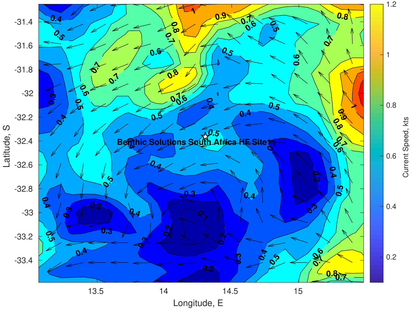
Surface Currents for Benthic Solutions South Africa HF Site1 at 13-Mar-2025 00:00:00
