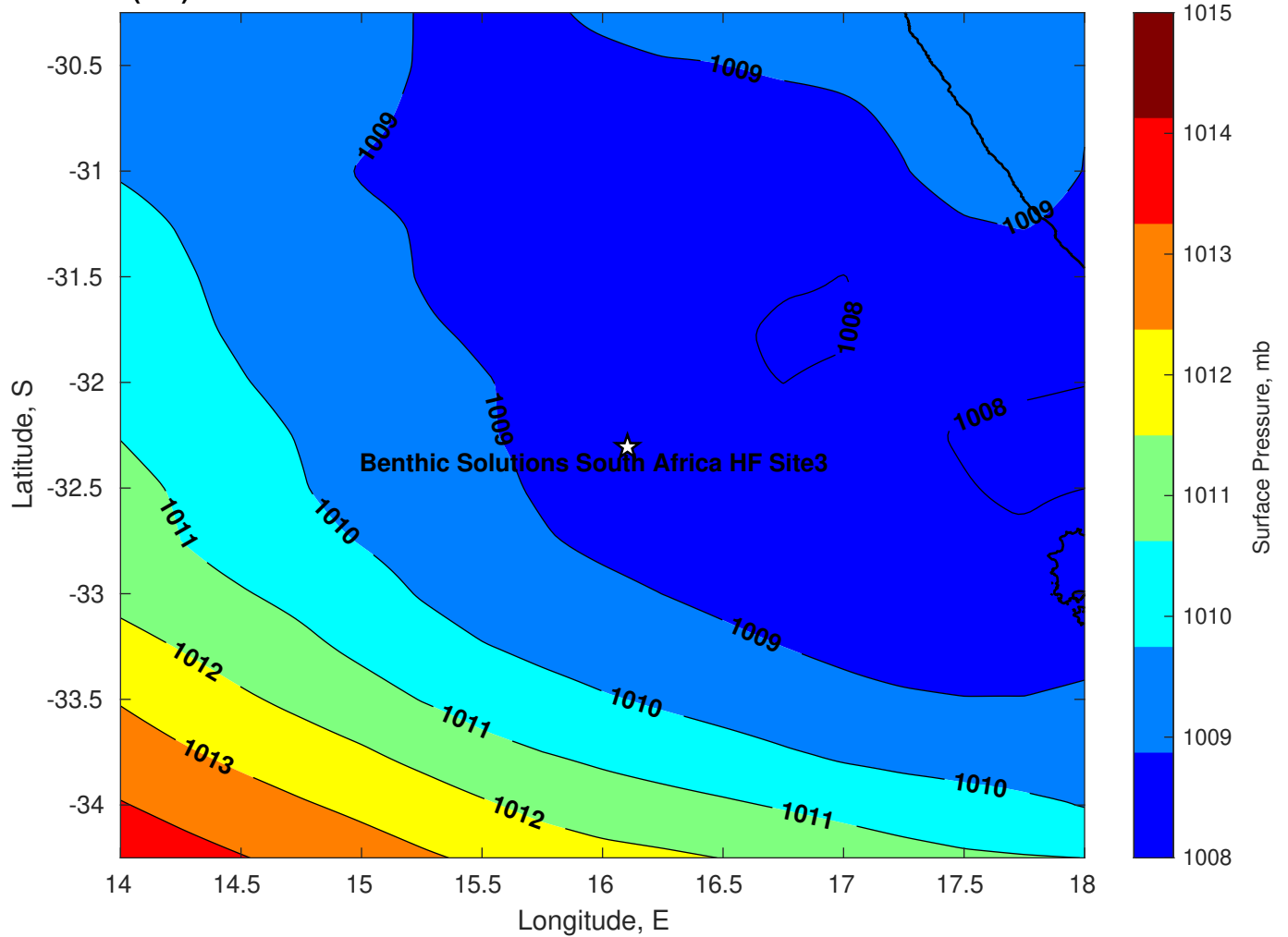
Surface Pressure (mb) for Benthic Solutions South Africa HF Site3 at 23-Mar-2025 00:00:00
