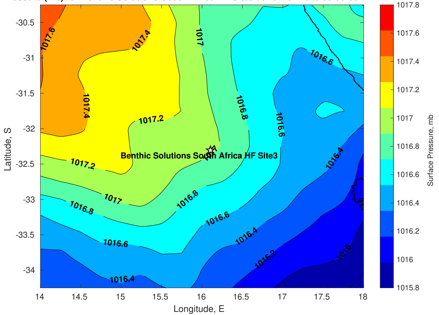
Surface Pressure (mb) for Benthic Solutions South Africa HF Site3 at 16-Mar-2025 00:00:00
