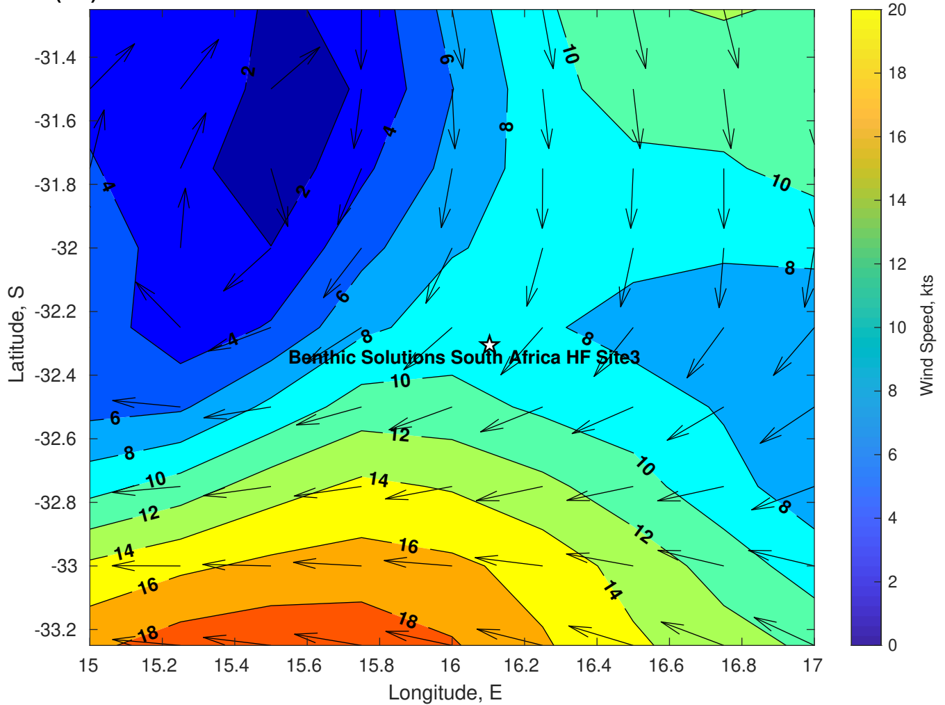
Winds (kts) for Benthic Solutions South Africa HF Site3 at 14-Mar-2025 09:00:00
