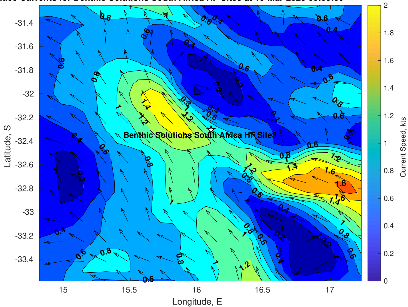
Surface Currents for Benthic Solutions South Africa HF Site3 at 13-Mar-2025 00:00:00
