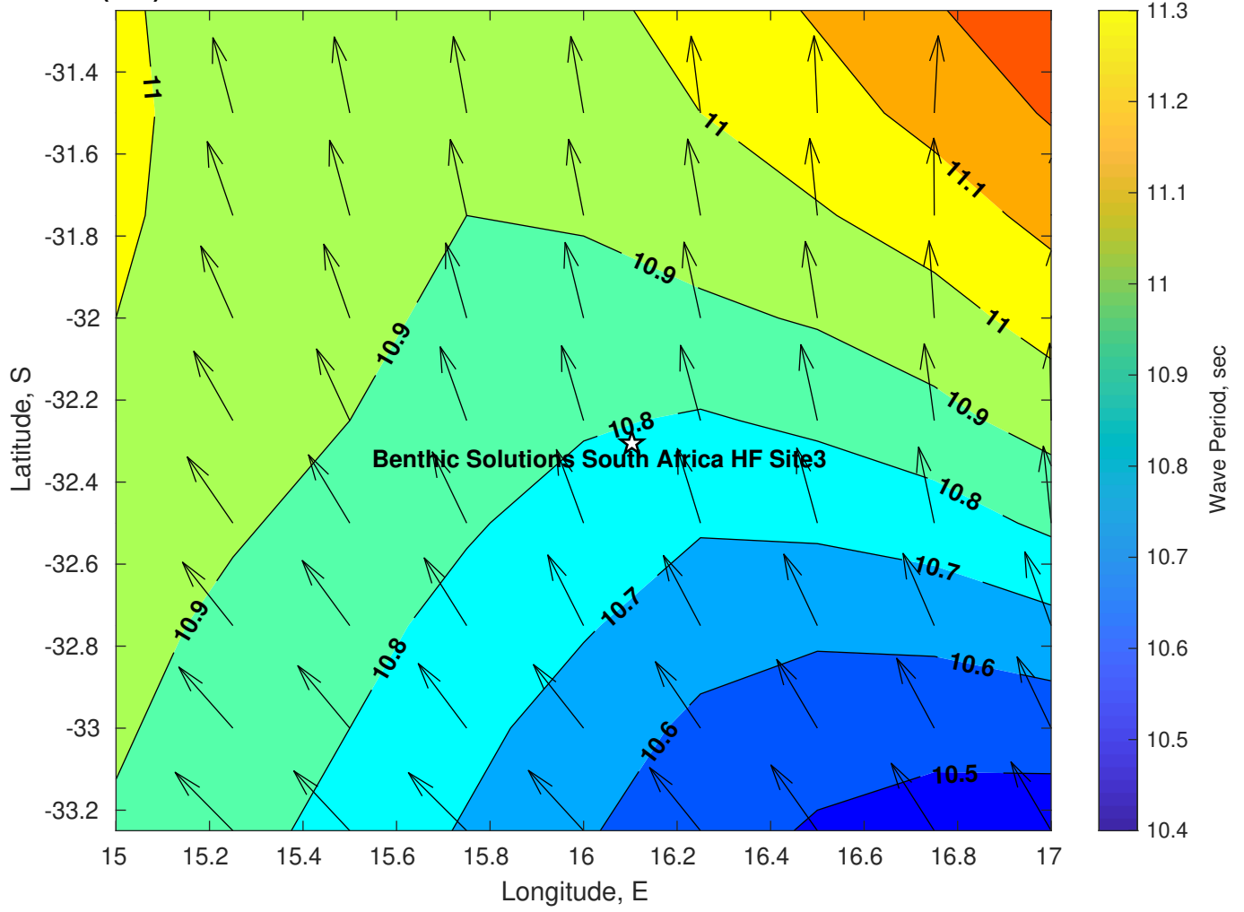
Wave Period (sec) for Benthic Solutions South Africa HF Site3 at 14-Mar-2025 09:00:00
