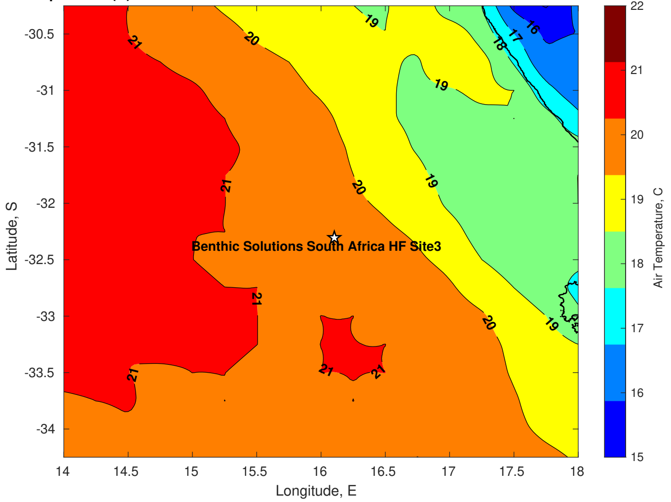
Air Temperature (C) for Benthic Solutions South Africa HF Site3 at 14-Mar-2025
