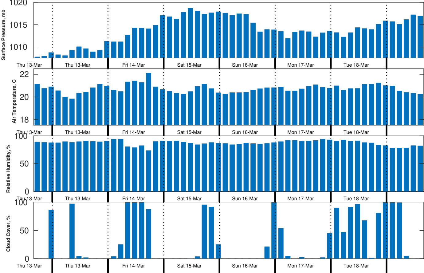
Met Forecast for Benthic Solutions South Africa HF Site3 from 13-Mar-2025 12:00:00 to 20-Mar-2025 12:00:00
