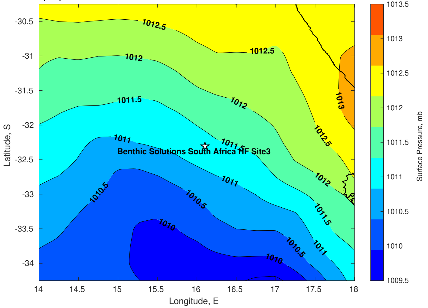
Surface Pressure (mb) for Benthic Solutions South Africa HF Site3 at 15-Mar-2025 00:00:00
