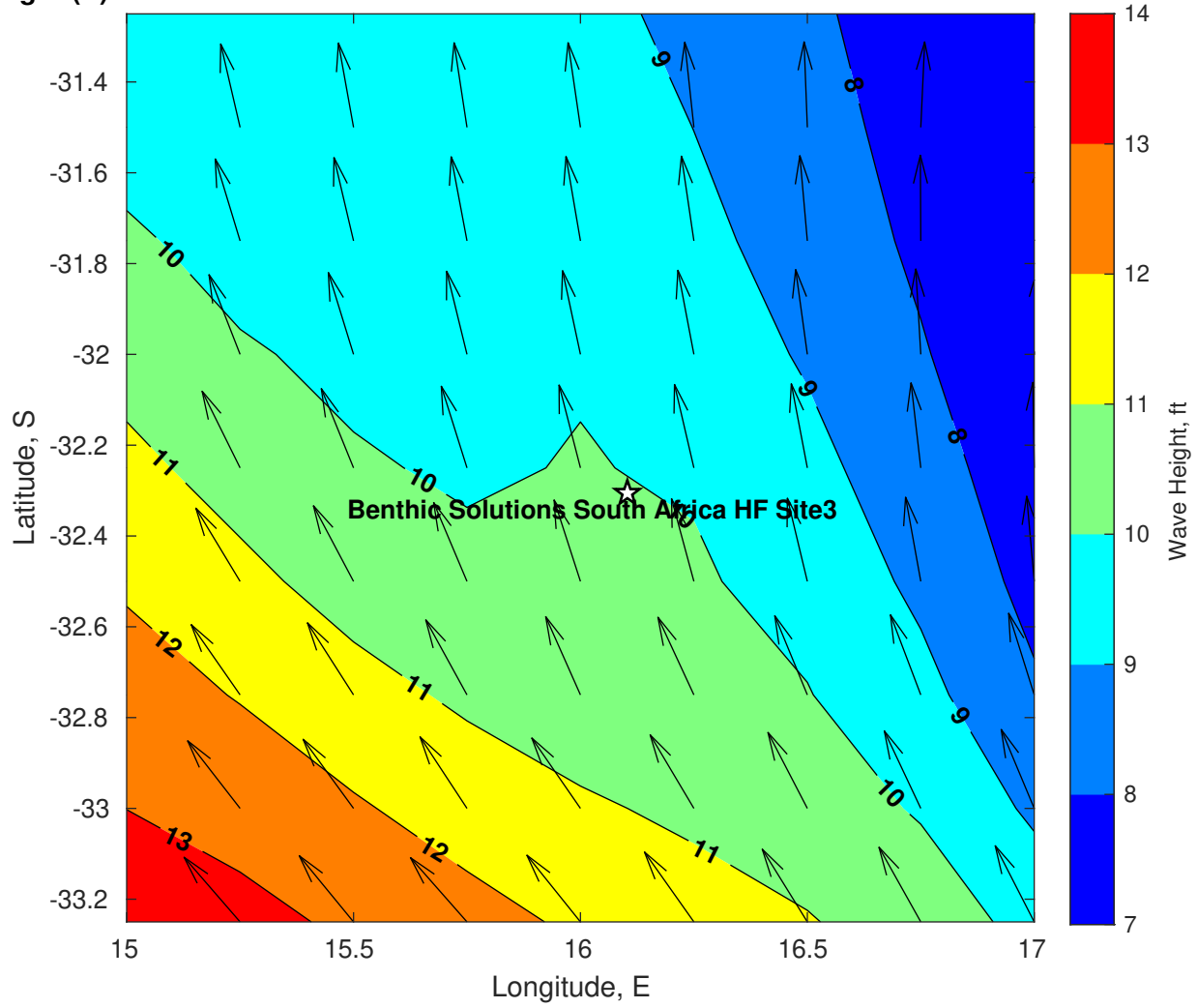
Wave Height (ft) for Benthic Solutions South Africa HF Site3 at 14-Mar-2025 09:00:00
