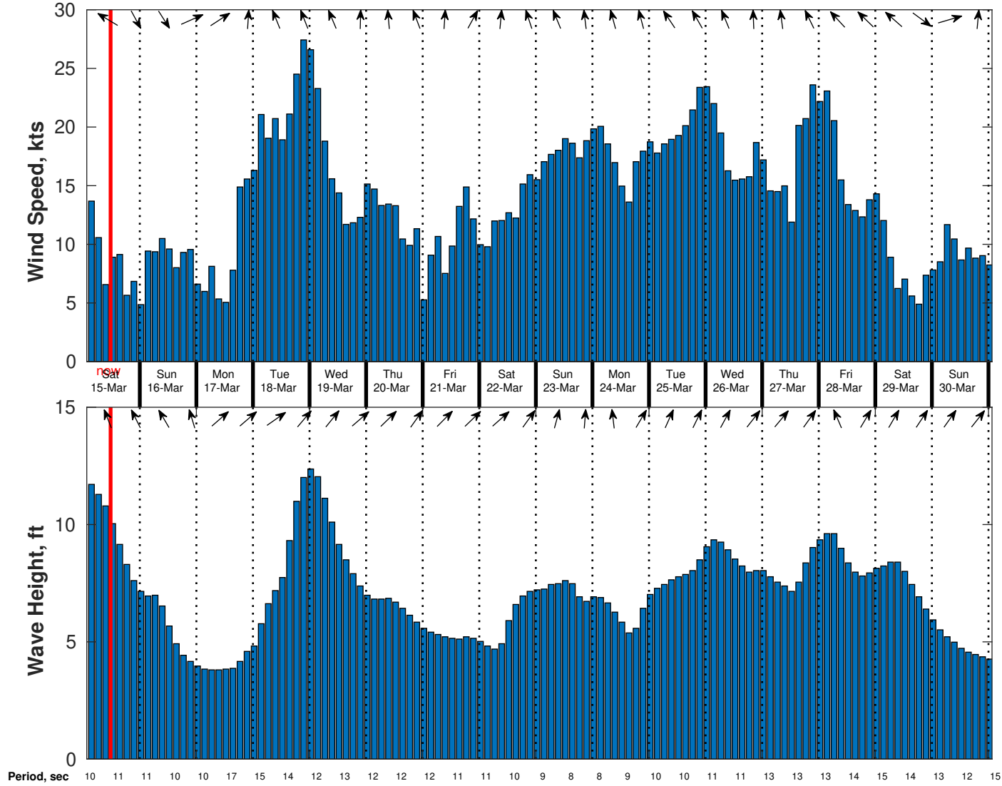
Wind & Wave Forecast for Benthic Solutions South Africa HF Site3 from 14-Mar-2025 02:00:00 to 30-Mar-2025 02:00:00
