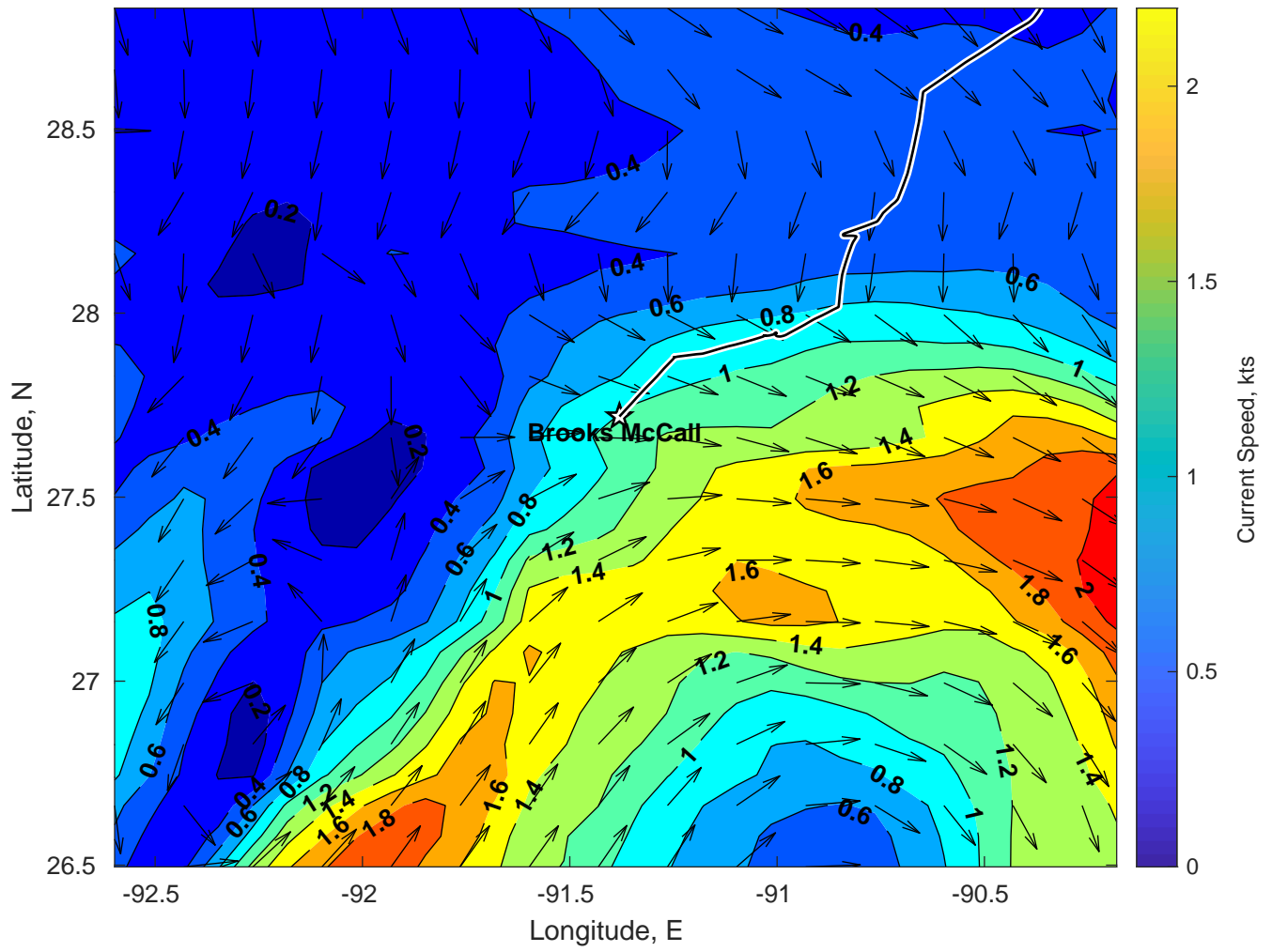
Surface Currents for Brooks McCall at 17-Mar-2025 00:00:00
