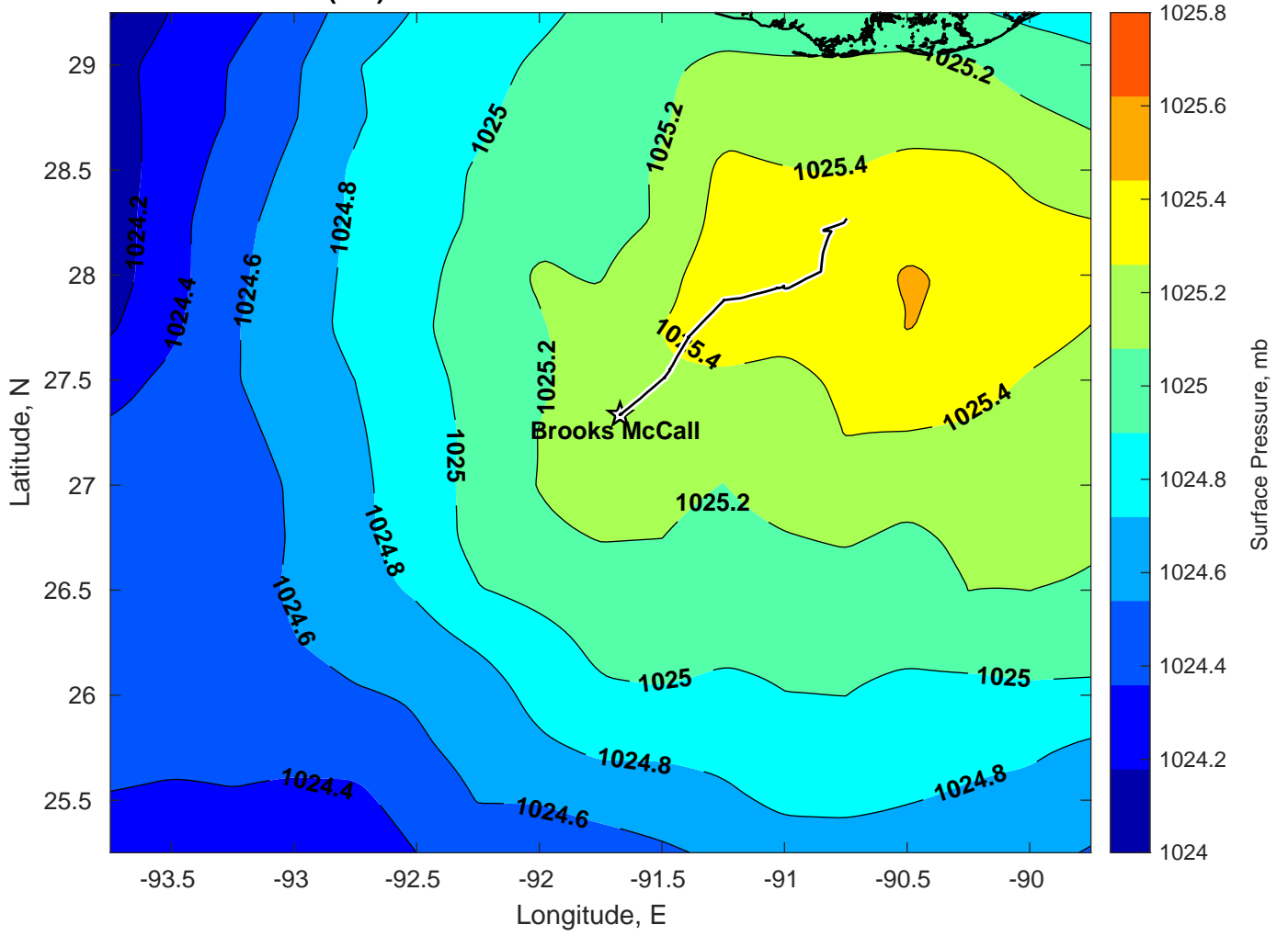
Surface Pressure (mb) for Brooks McCall at 18-Mar-2025 00:00:00
