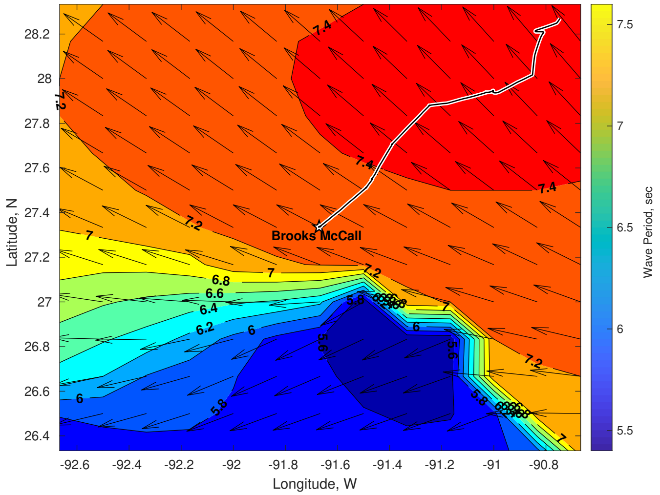
Wave Period (sec) for Brooks McCall at 18-Mar-2025 09:00:00
