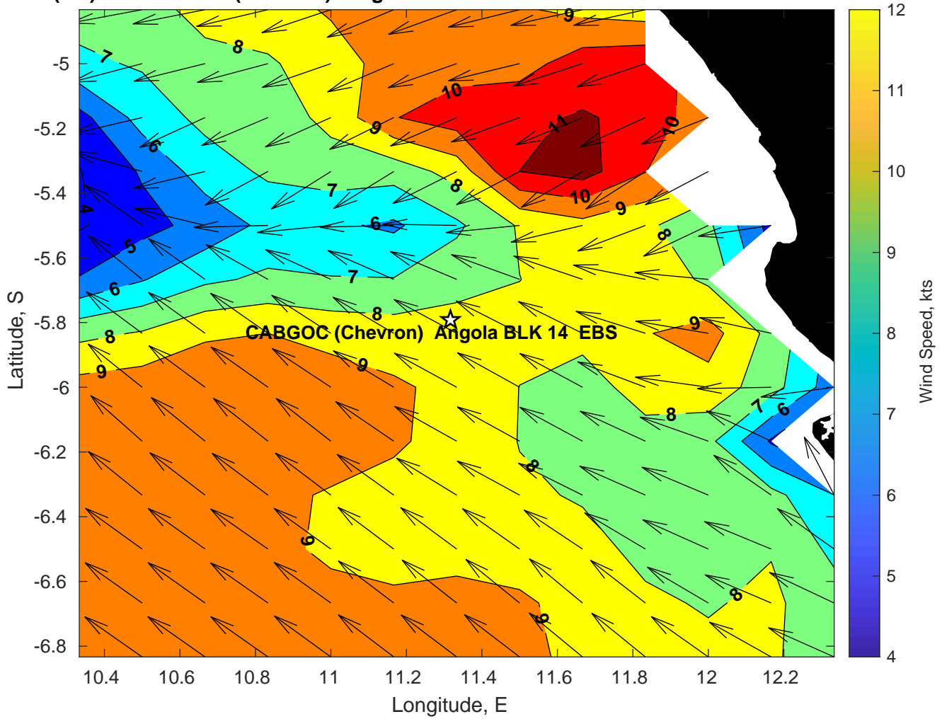
Winds (kts) for CABGOC (Chevron) Angola BLK 14 EBS at 14-Mar-2025 09:00:00
