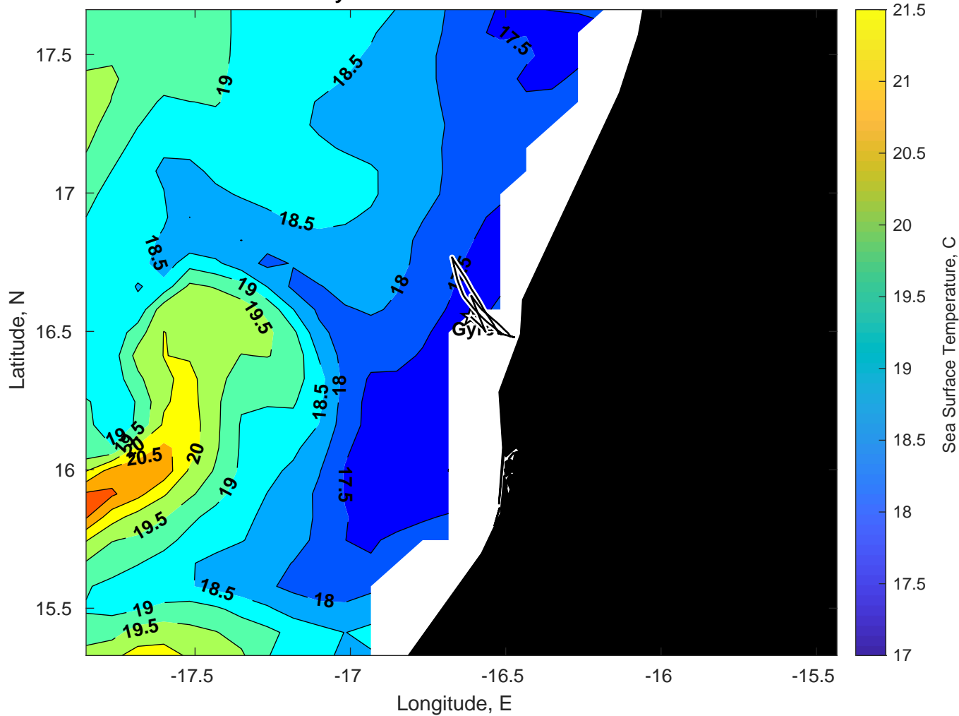
SST for Gyre at 17-Mar-2025 00:00:00
