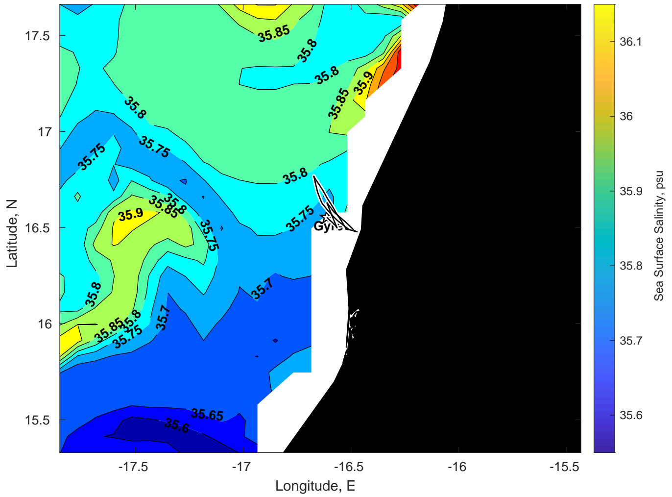
Surface Salinity for Gyre at 17-Mar-2025 00:00:00
