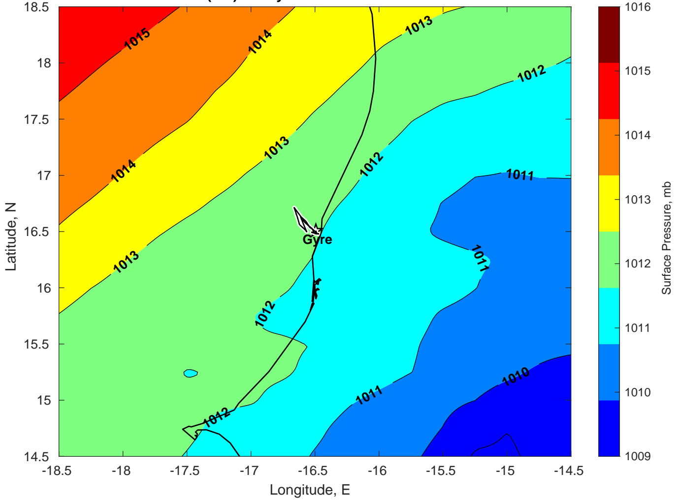
Surface Pressure (mb) for Gyre at 18-Mar-2025 00:00:00
