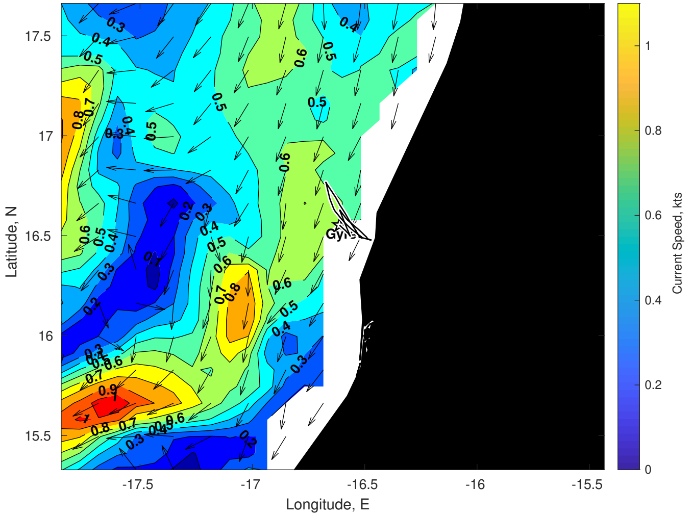
Surface Currents for Gyre at 17-Mar-2025 00:00:00
