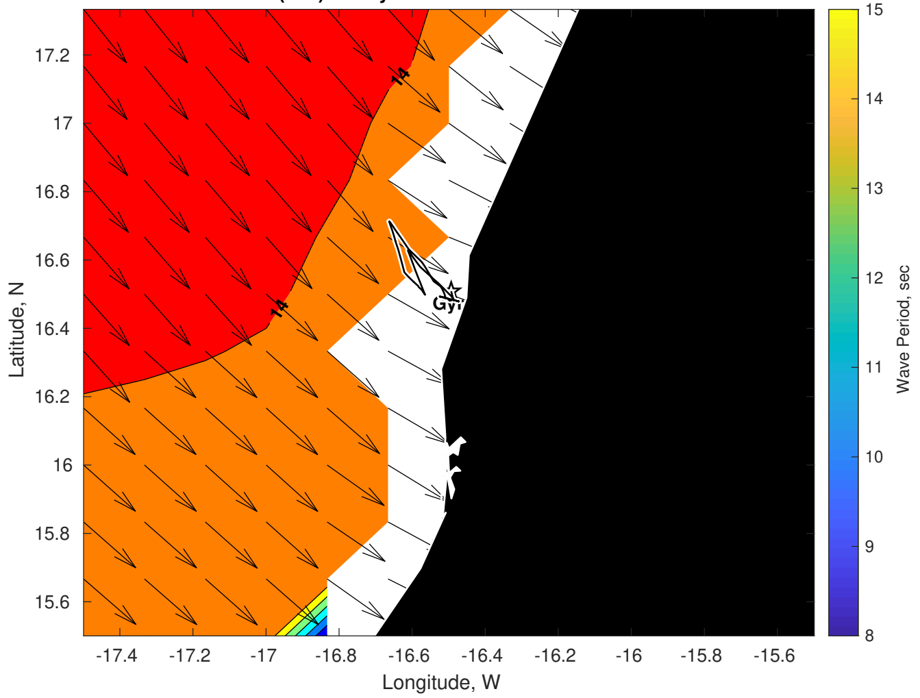
Wave Period (sec) for Gyre at 18-Mar-2025 09:00:00
