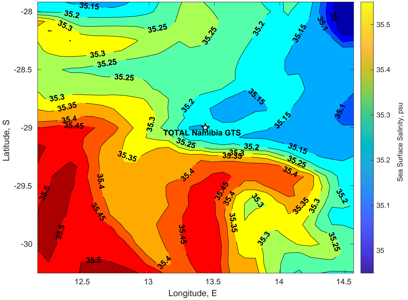
Surface Salinity for TOTAL Namibia GTS at 13-Mar-2025 00:00:00
