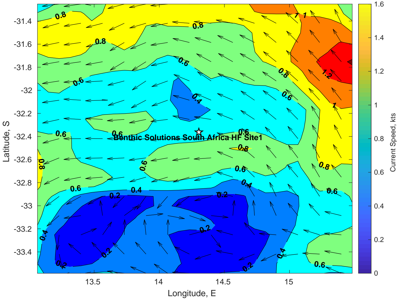
Surface Currents for Benthic Solutions South Africa HF Site1 at 18-Mar-2025 00:00:00
