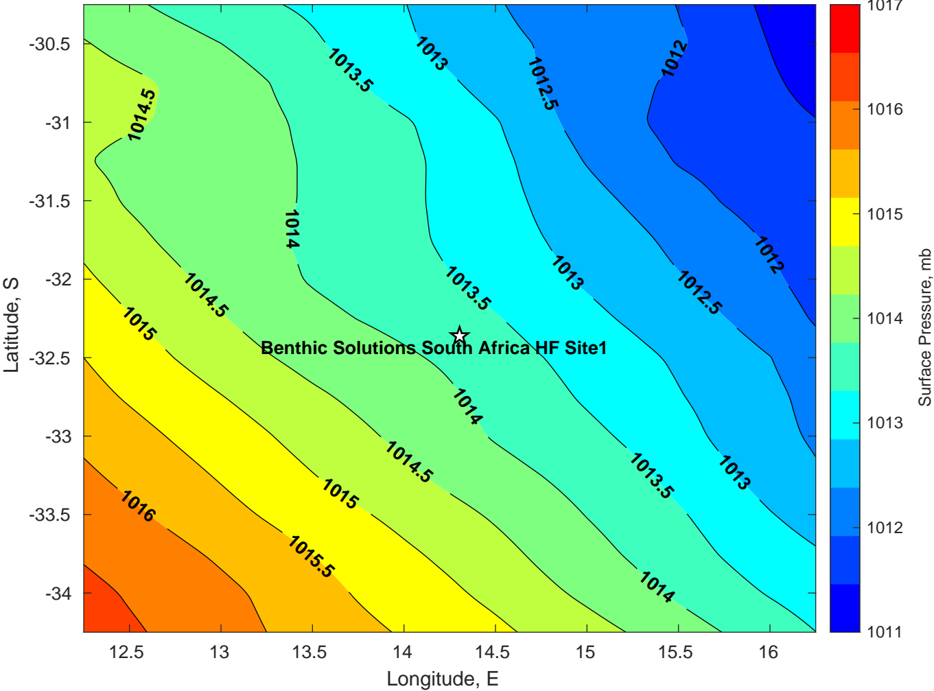
Surface Pressure (mb) for Benthic Solutions South Africa HF Site1 at 19-Mar-2025 00:00:00
