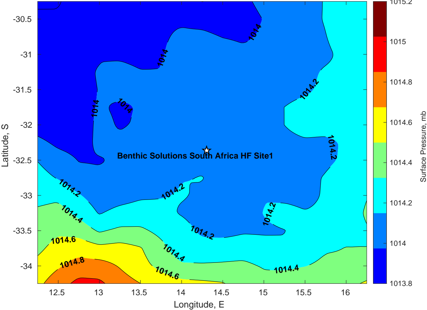
Surface Pressure (mb) for Benthic Solutions South Africa HF Site1 at 21-Mar-2025 00:00:00
