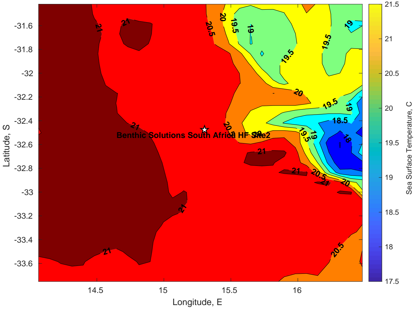
SST for Benthic Solutions South Africa HF Site2 at 18-Mar-2025 00:00:00
