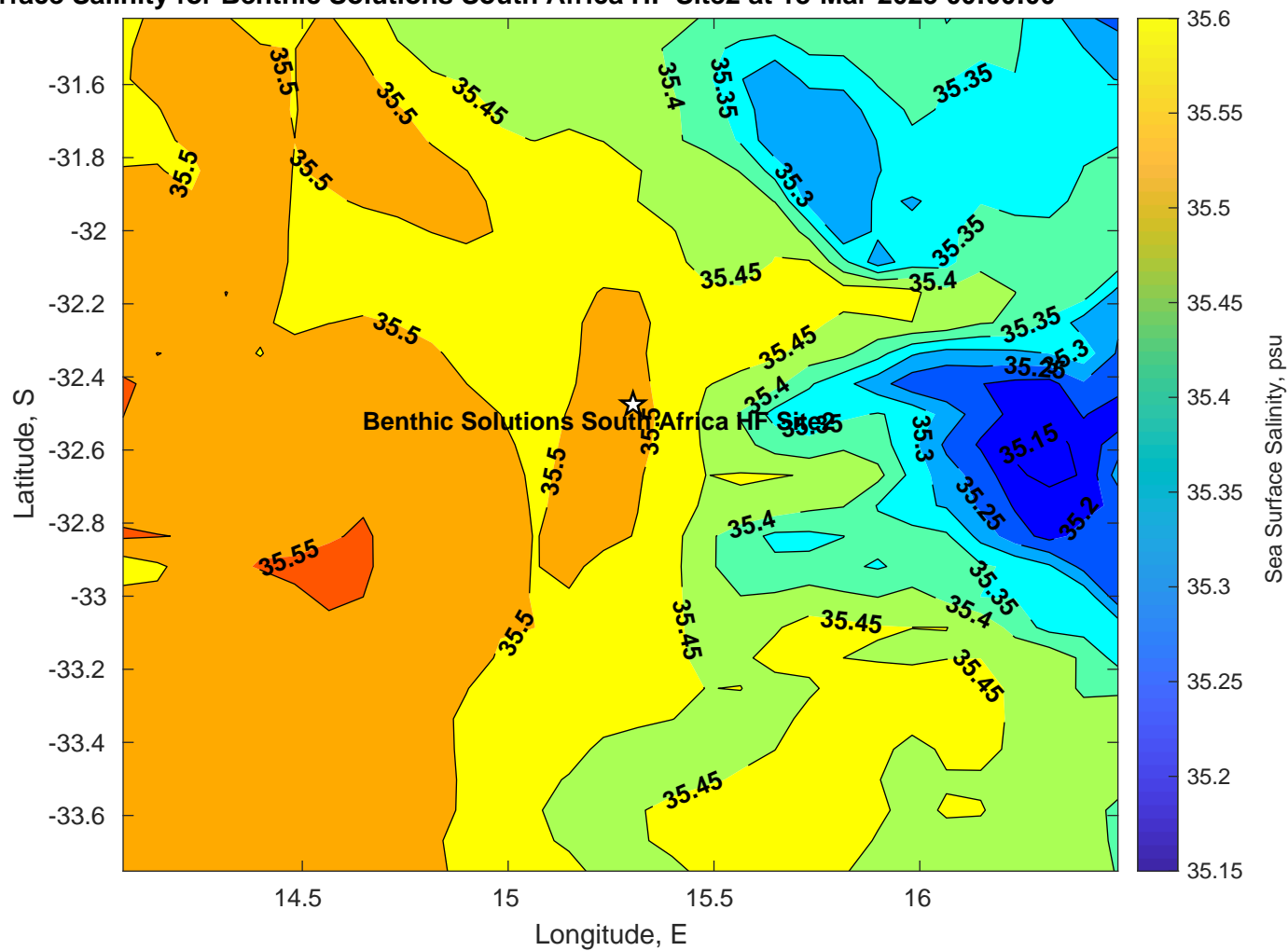
Surface Salinity for Benthic Solutions South Africa HF Site2 at 18-Mar-2025 00:00:00
