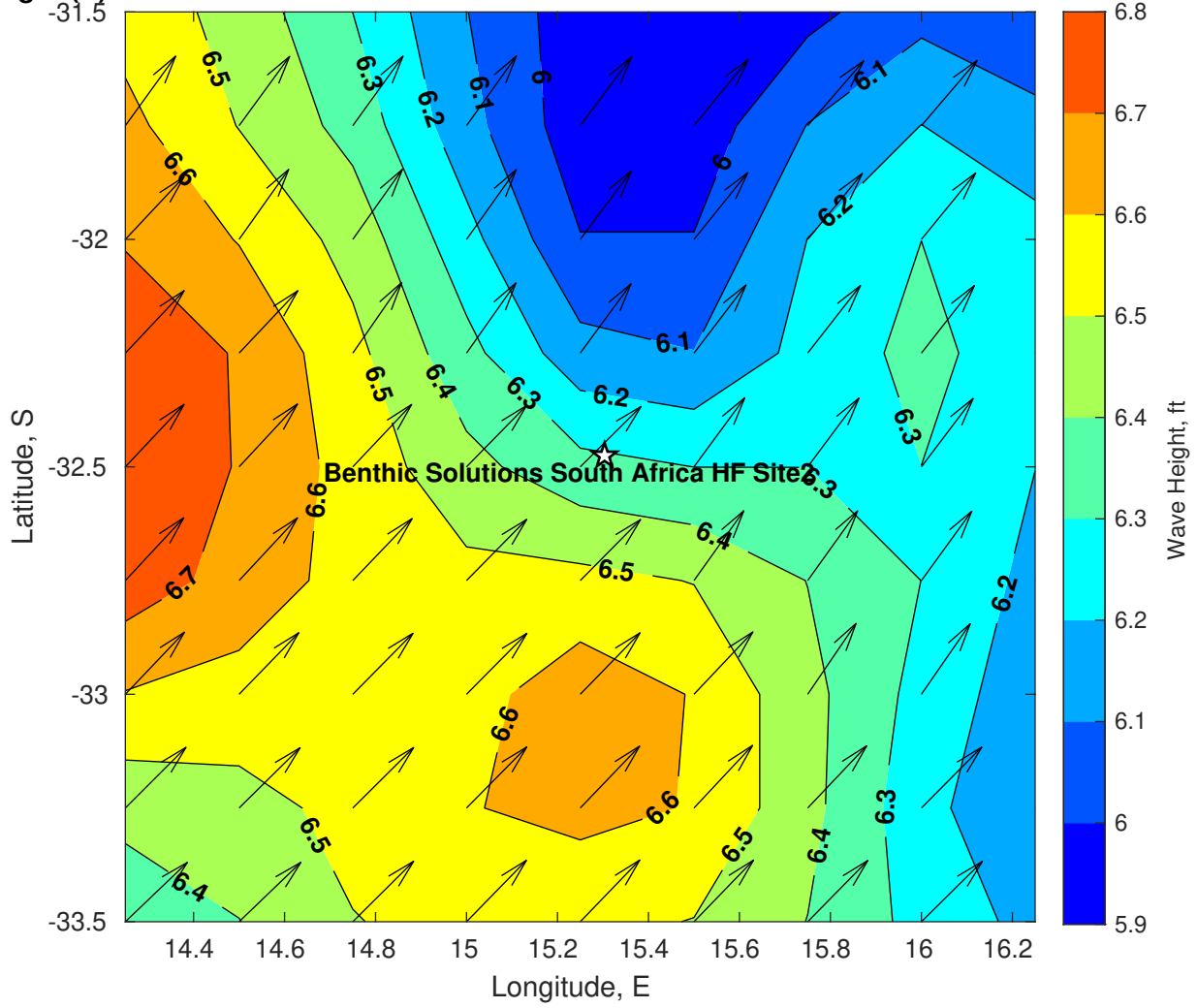
Wave Height (ft) for Benthic Solutions South Africa HF Site2 at 19-Mar-2025 09:00:00
