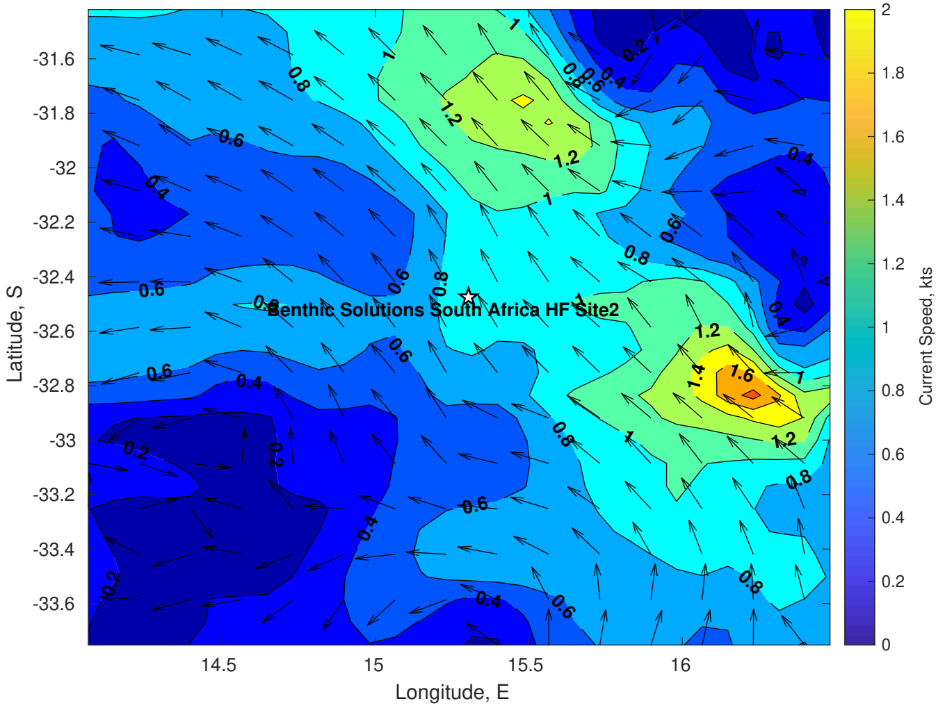
Surface Currents for Benthic Solutions South Africa HF Site2 at 18-Mar-2025 00:00:00
