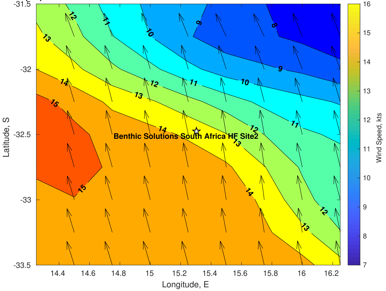
Winds (kts) for Benthic Solutions South Africa HF Site2 at 19-Mar-2025 09:00:00
