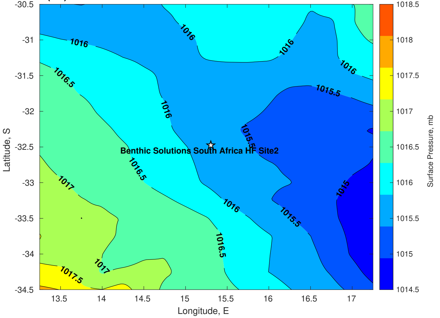
Surface Pressure (mb) for Benthic Solutions South Africa HF Site2 at 20-Mar-2025 00:00:00
