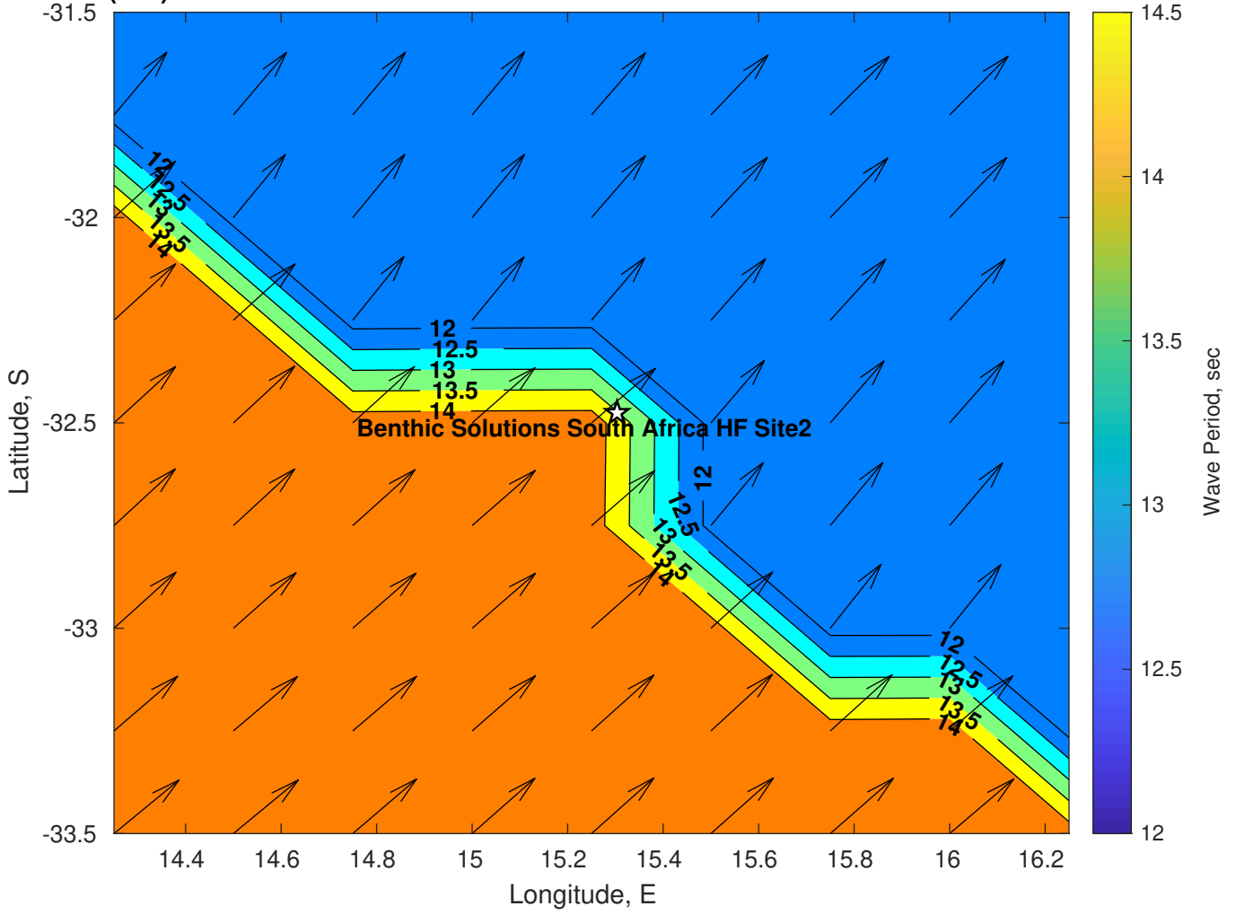
Wave Period (sec) for Benthic Solutions South Africa HF Site2 at 19-Mar-2025 09:00:00
