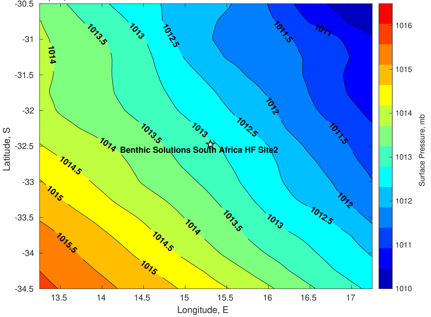
Surface Pressure (mb) for Benthic Solutions South Africa HF Site2 at 19-Mar-2025 00:00:00
