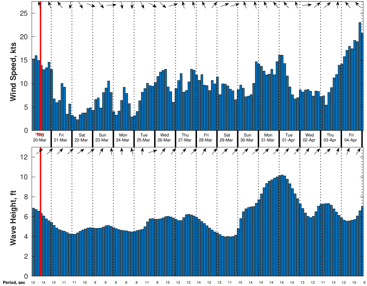
Wind & Wave Forecast for Benthic Solutions South Africa HF Site2 from 19-Mar-2025 02:00:00 to 04-Apr-2025 02:00:00
