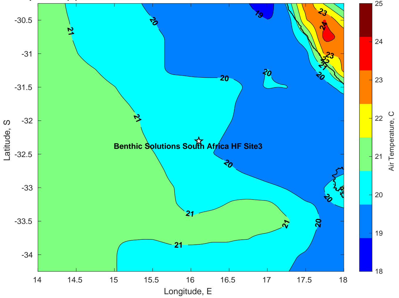
Air Temperature (C) for Benthic Solutions South Africa HF Site3 at 19-Mar-2025
