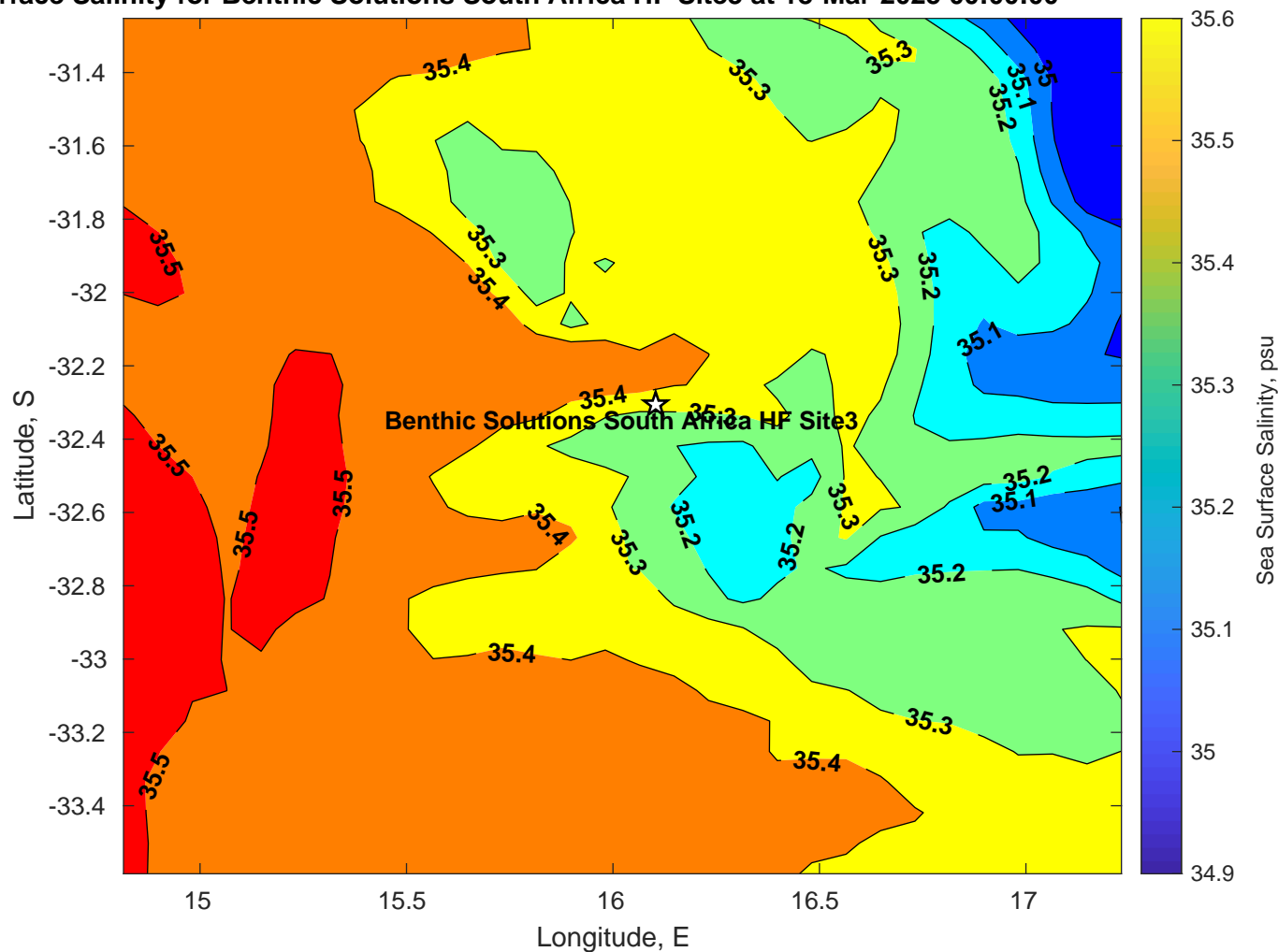
Surface Salinity for Benthic Solutions South Africa HF Site3 at 18-Mar-2025 00:00:00
