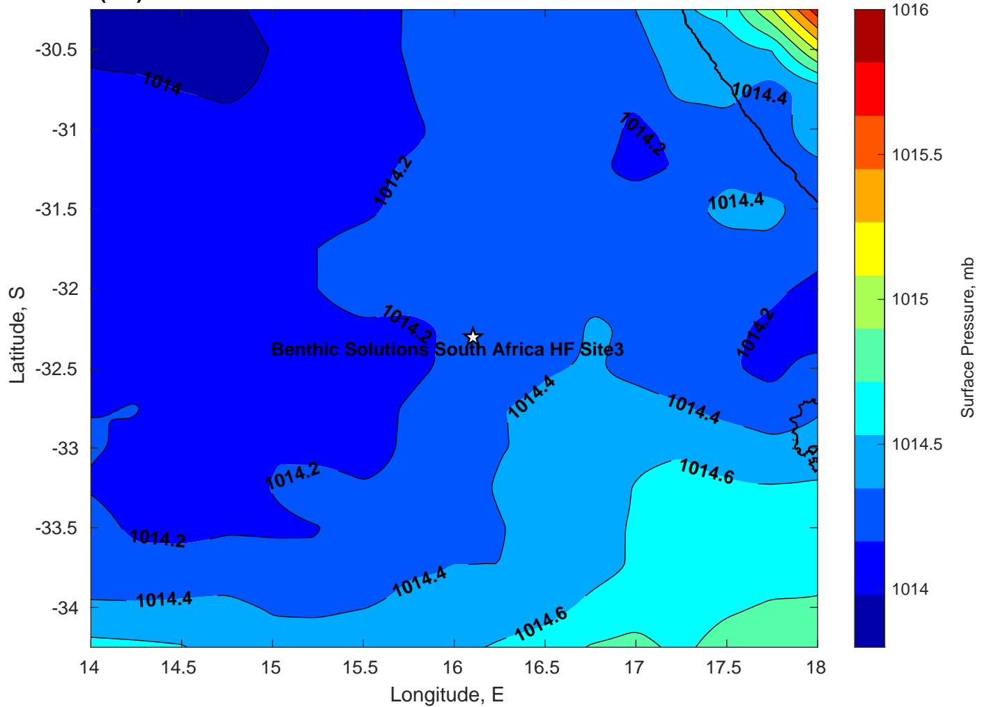
Surface Pressure (mb) for Benthic Solutions South Africa HF Site3 at 21-Mar-2025 00:00:00
