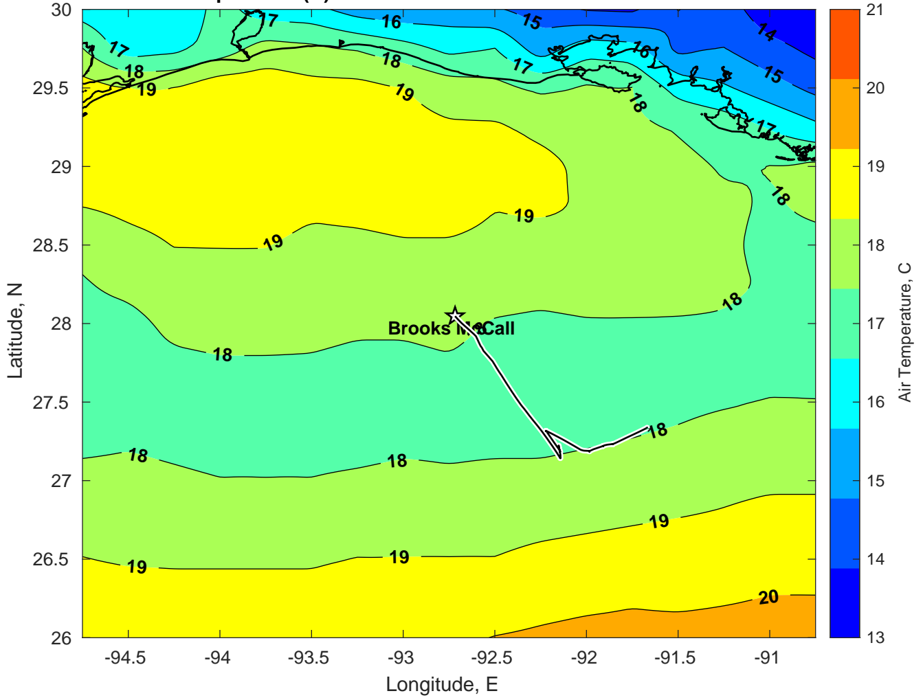
Air Temperature (C) for Brooks McCall at 19-Mar-2025
