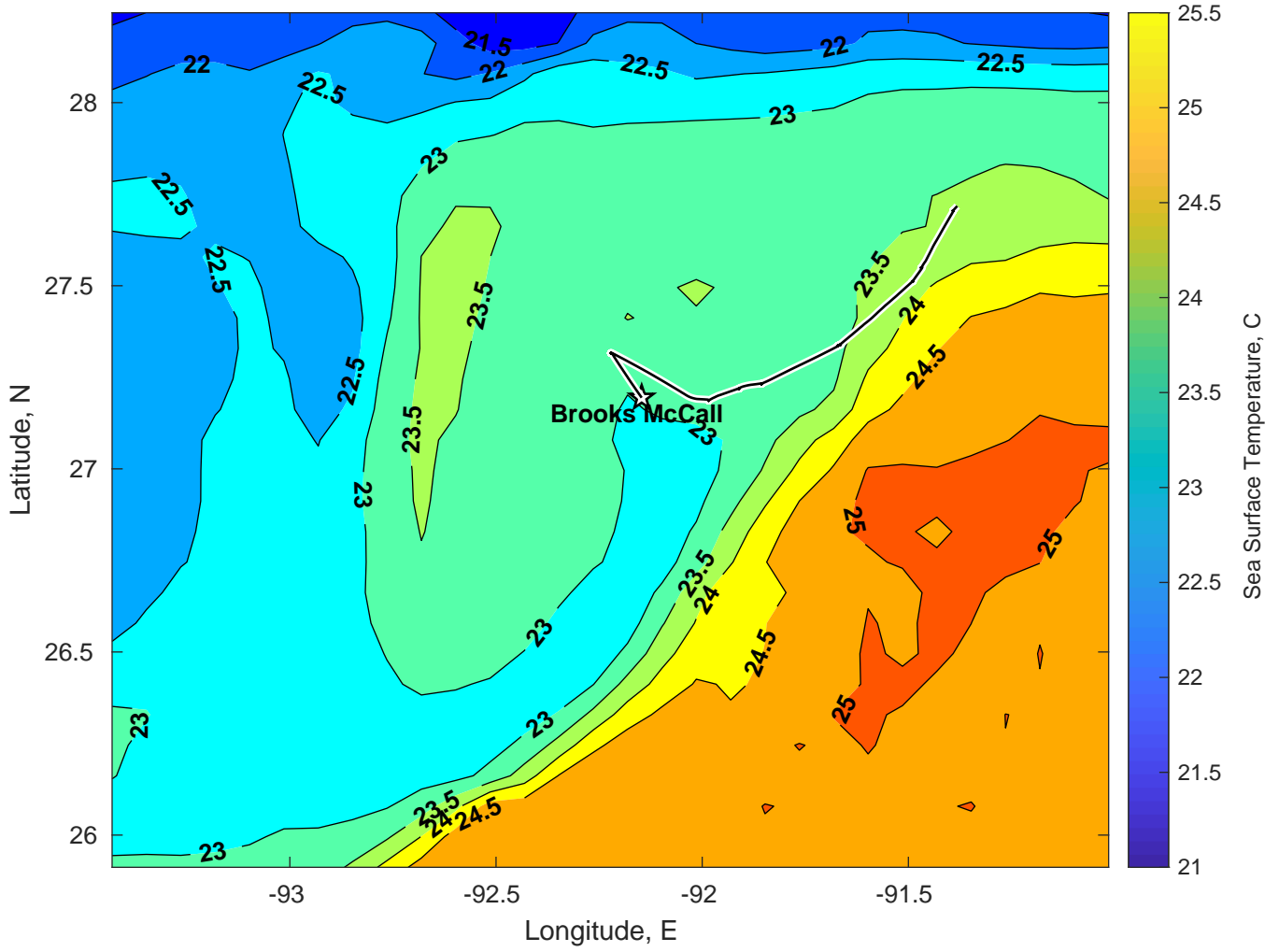
SST for Brooks McCall at 18-Mar-2025 00:00:00
