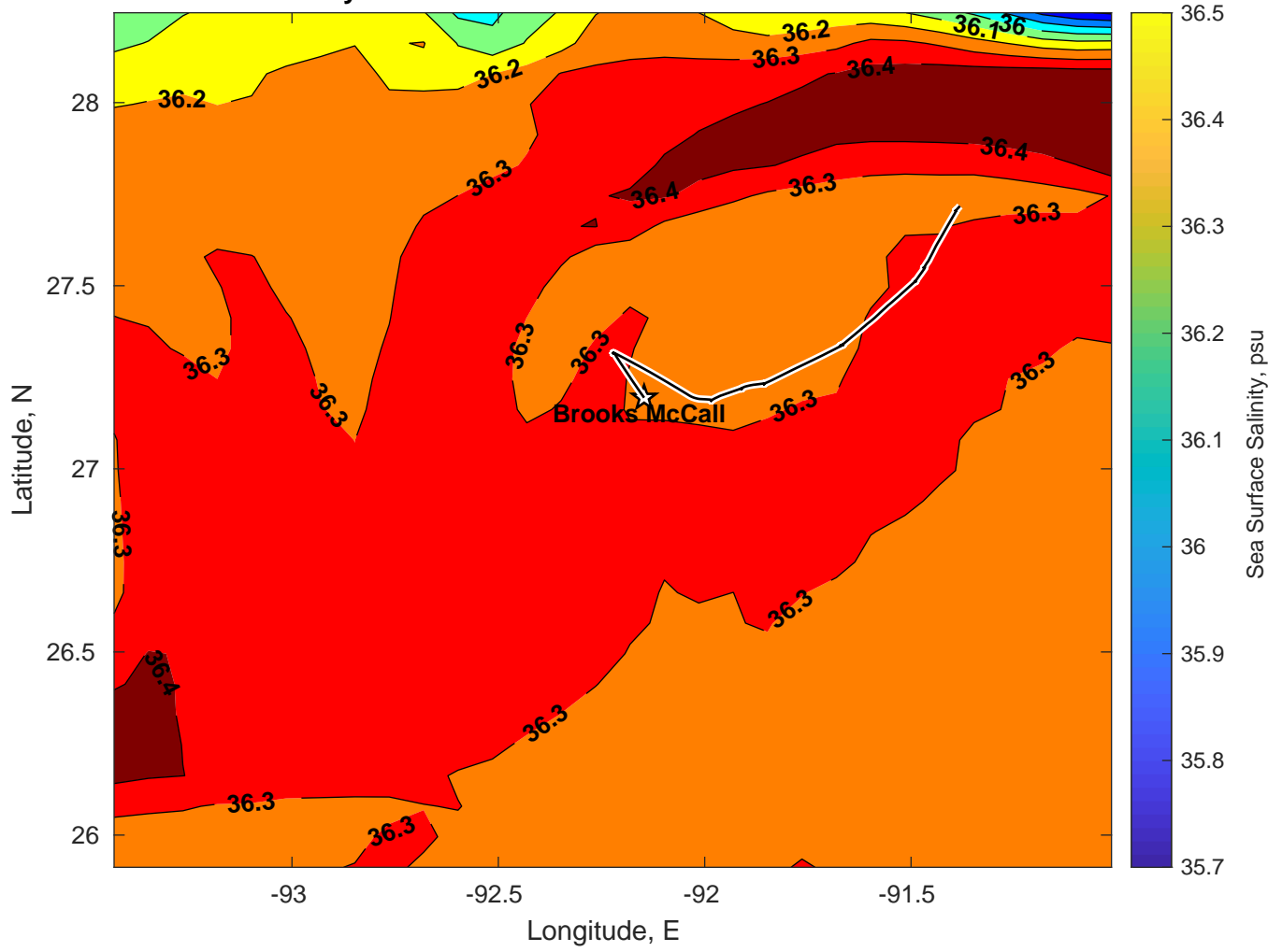
Surface Salinity for Brooks McCall at 18-Mar-2025 00:00:00
