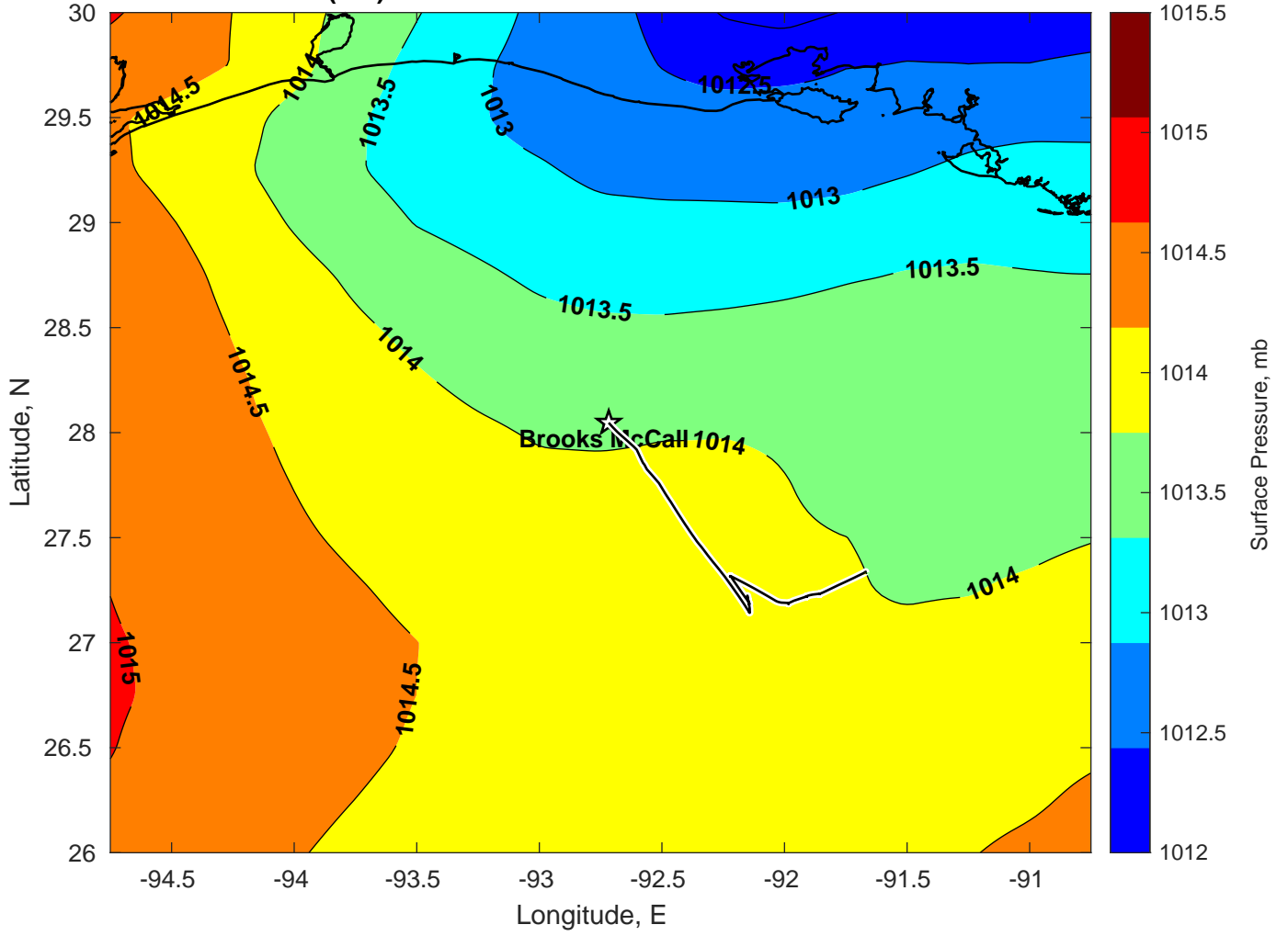
Surface Pressure (mb) for Brooks McCall at 20-Mar-2025 00:00:00
