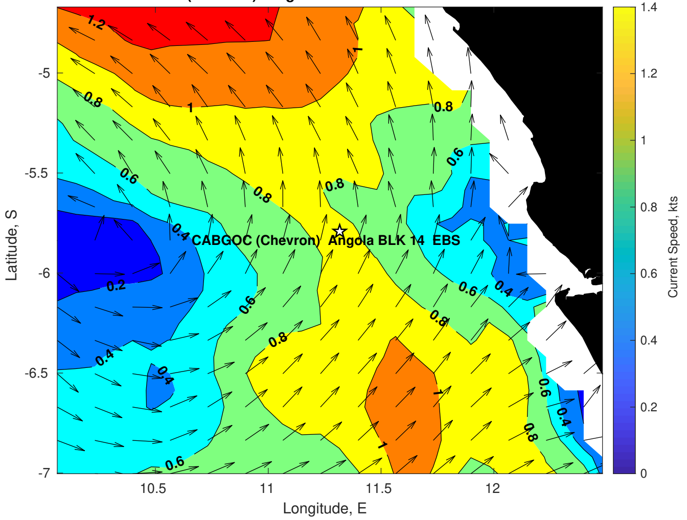
Surface Currents for CABGOC (Chevron) Angola BLK 14 EBS at 18-Mar-2025 00:00:00
