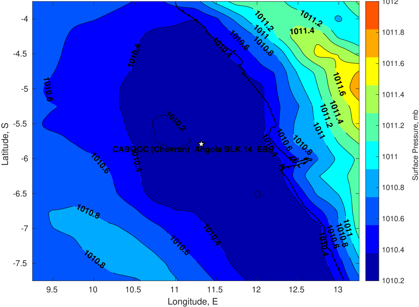
Surface Pressure (mb) for CABGOC (Chevron) Angola BLK 14 EBS at 19-Mar-2025 00:00:00
