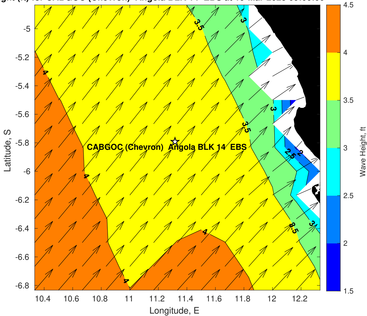
Wave Height (ft) for CABGOC (Chevron) Angola BLK 14 EBS at 19-Mar-2025 09:00:00
