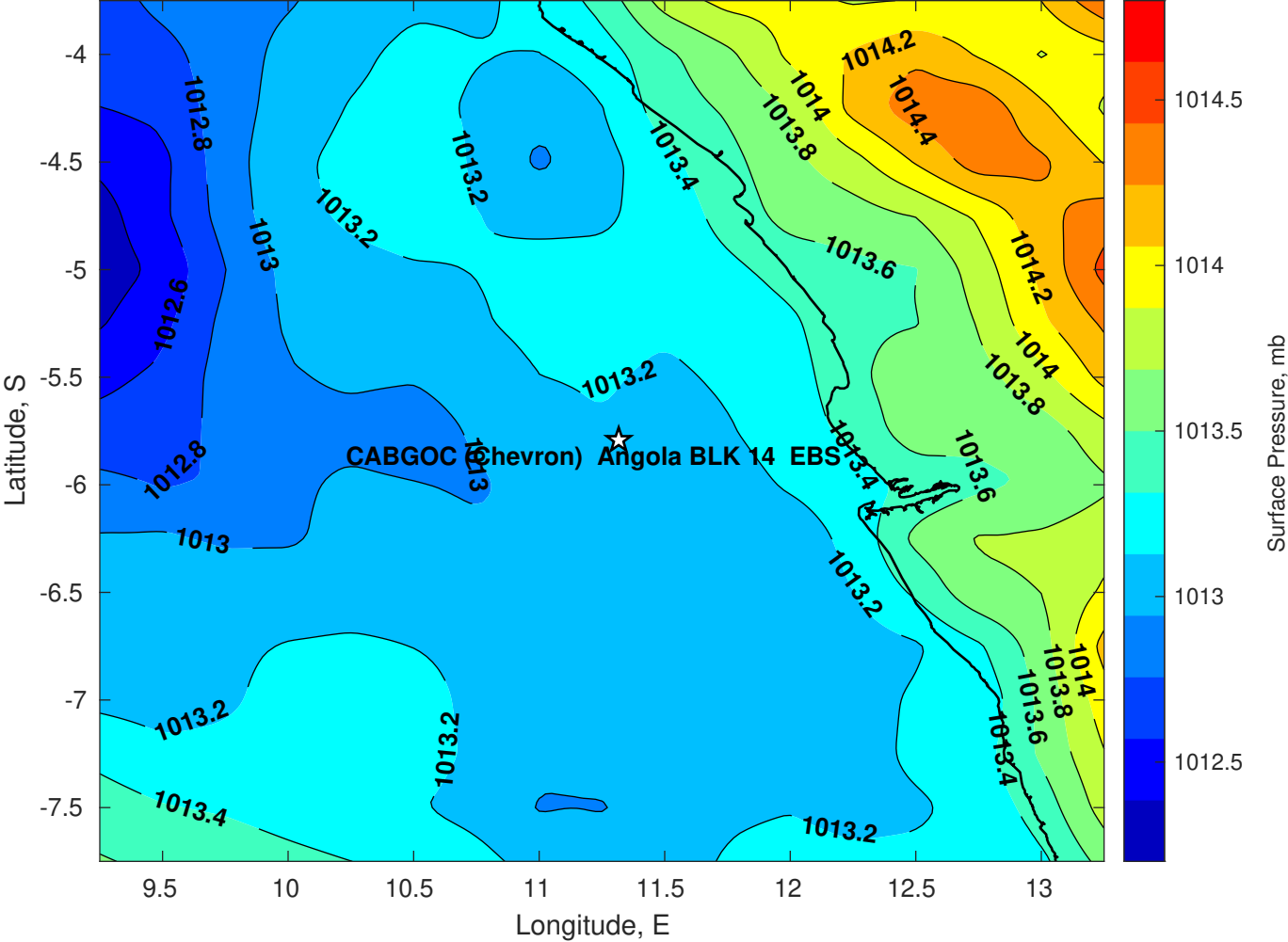
Surface Pressure (mb) for CABGOC (Chevron) Angola BLK 14 EBS at 21-Mar-2025 00:00:00
