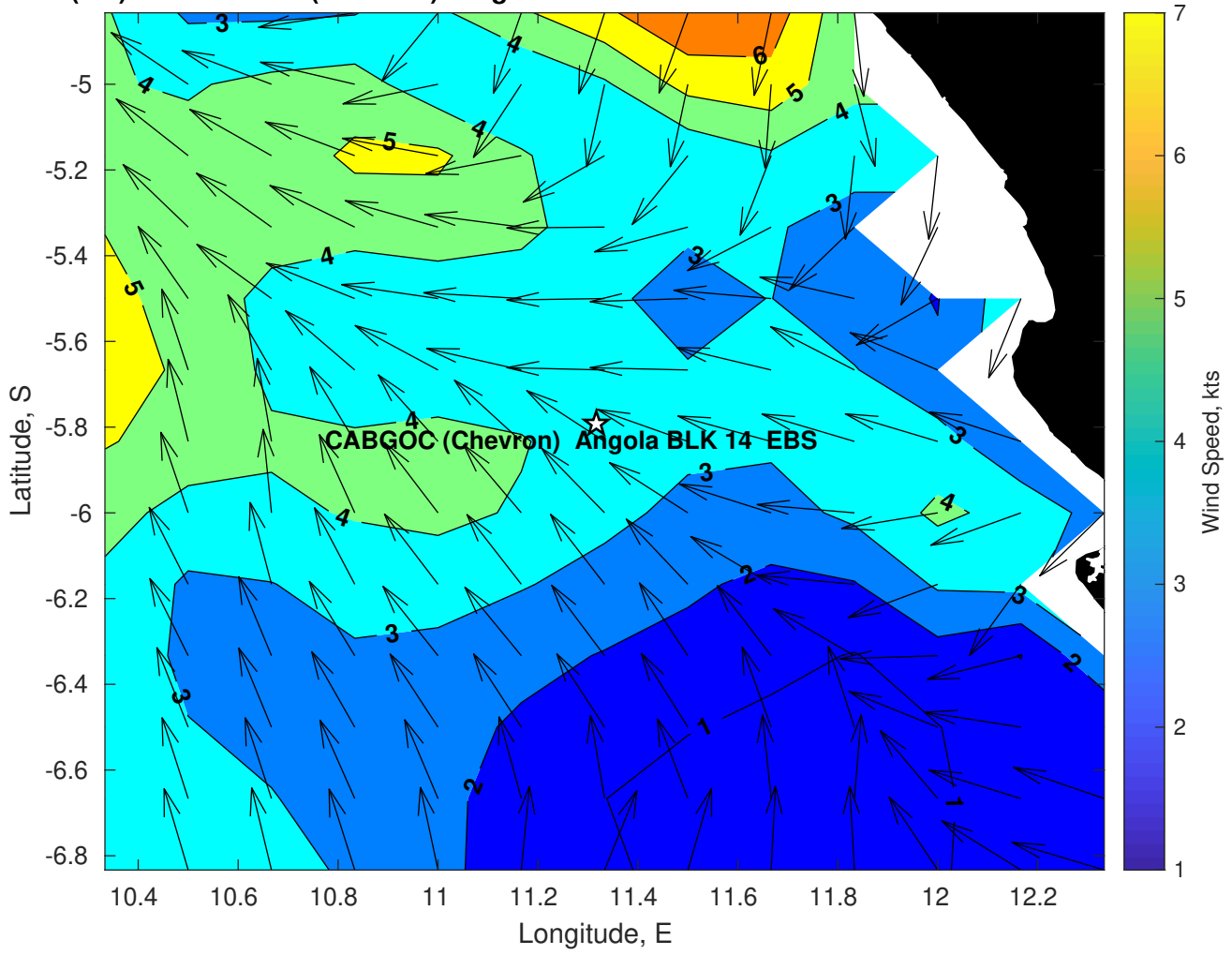
Winds (kts) for CABGOC (Chevron) Angola BLK 14 EBS at 19-Mar-2025 09:00:00
