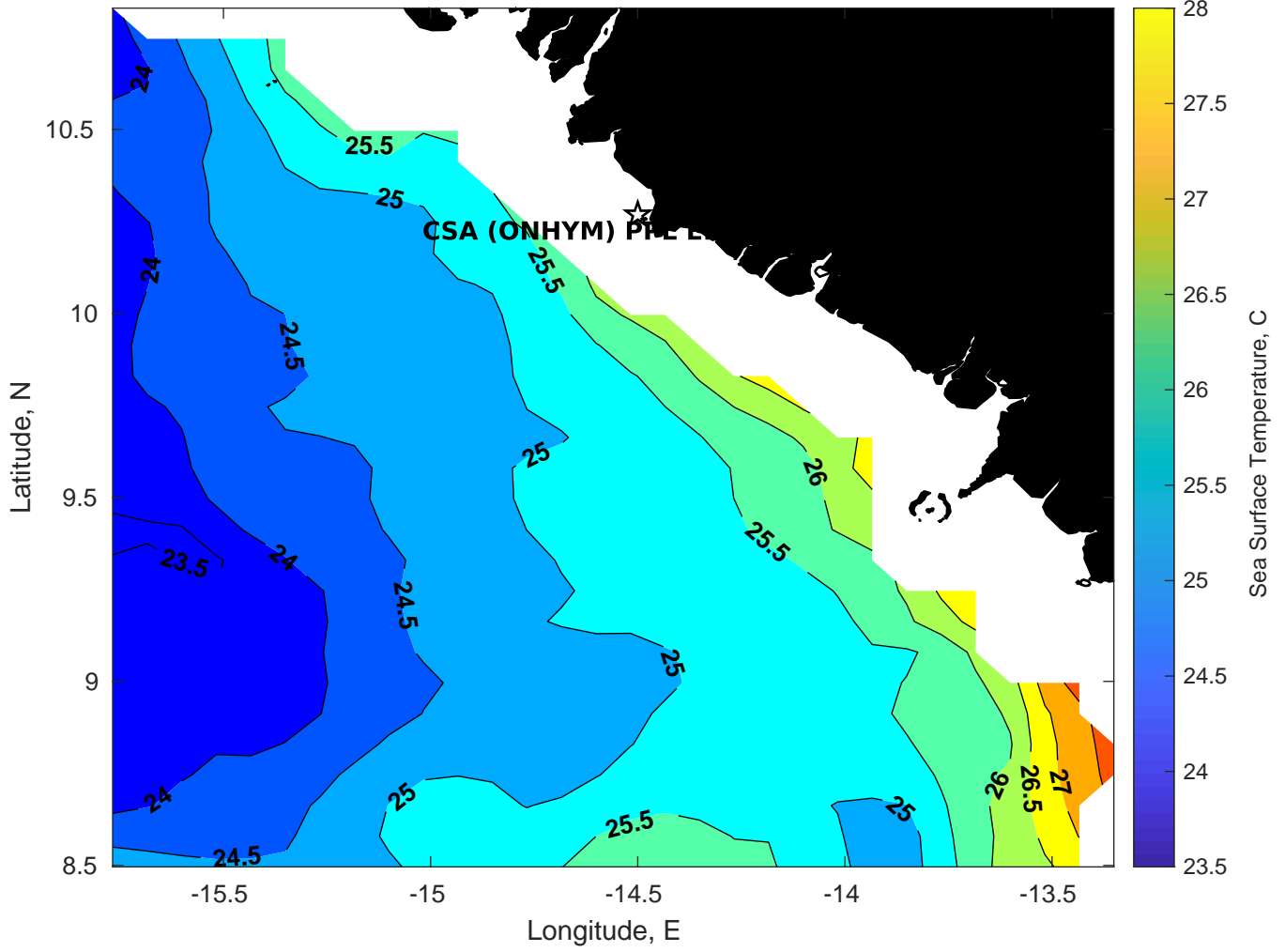
SST for CSA (ONHYM) PPL EBS - Guinea at 18-Mar-2025 00:00:00
