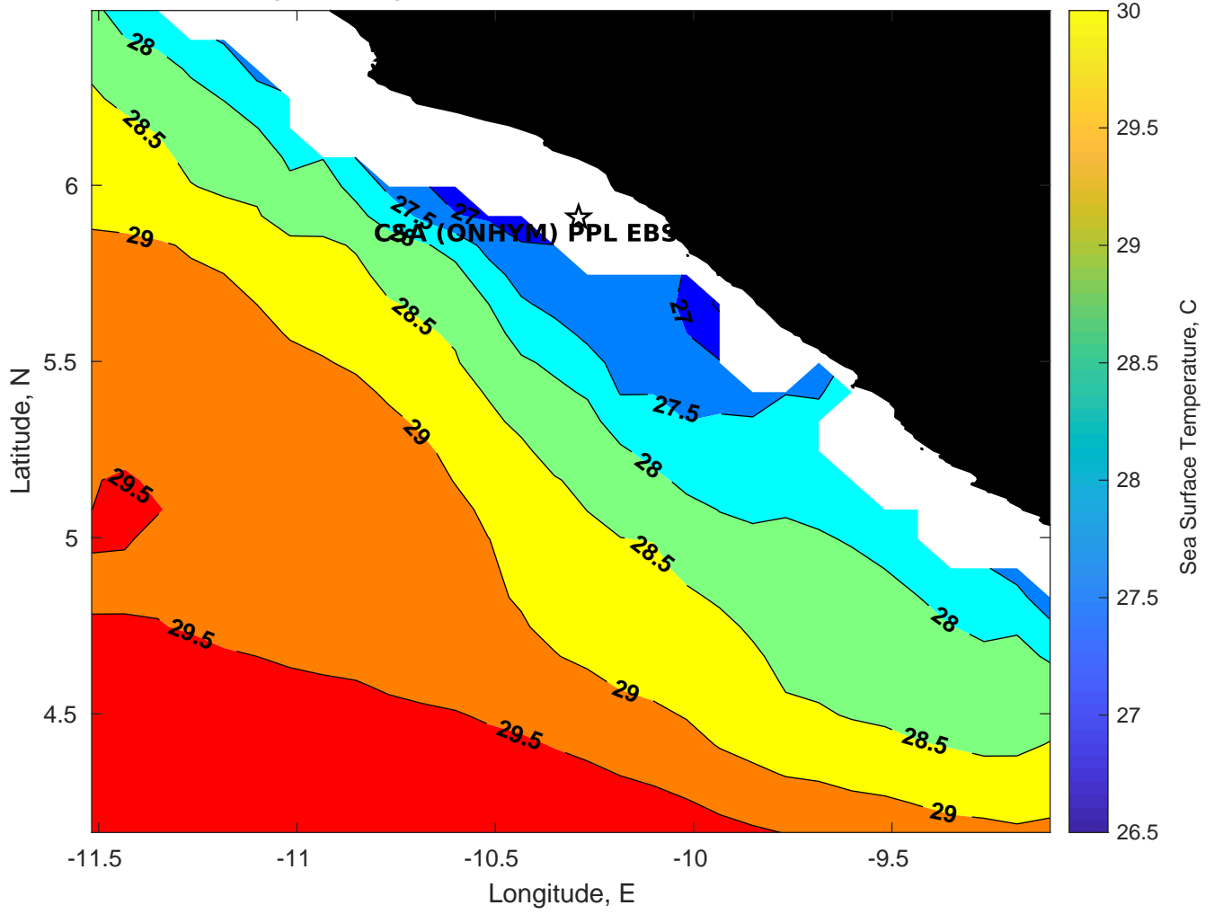
SST for CSA (ONHYM) PPL EBS - Liberia at 18-Mar-2025 00:00:00
