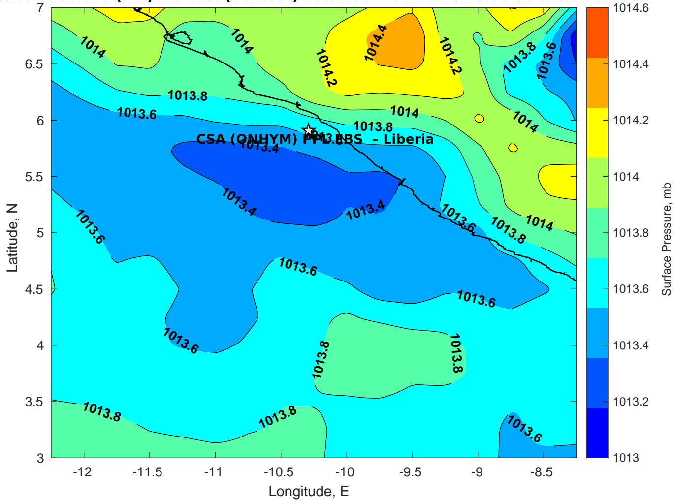
Surface Pressure (mb) for CSA (ONHYM) PPL EBS - Liberia at 21-Mar-2025 00:00:00
