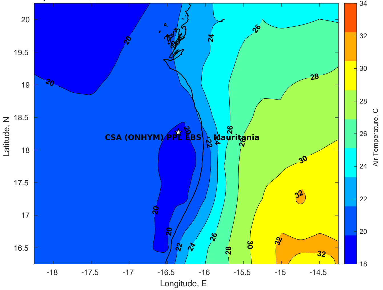
Air Temperature (C) for CSA (ONHYM) PPL EBS - Mauritania at 19-Mar-2025
