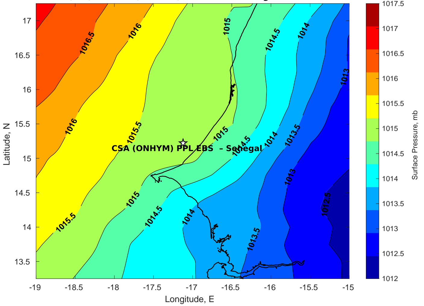
Surface Pressure (mb) for CSA (ONHYM) PPL EBS - Senegal at 21-Mar-2025 00:00:00
