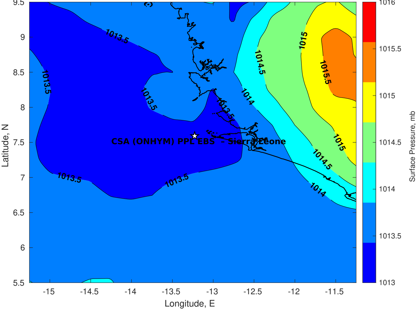
Surface Pressure (mb) for CSA (ONHYM) PPL EBS - Sierra Leone at 20-Mar-2025 00:00:00
