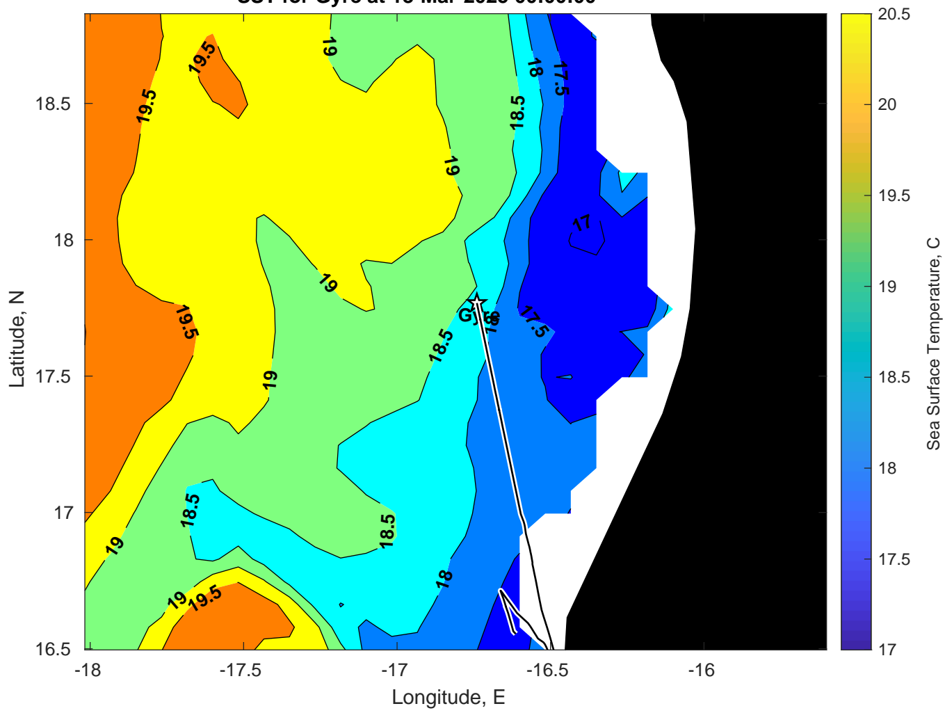
SST for Gyre at 18-Mar-2025 00:00:00
