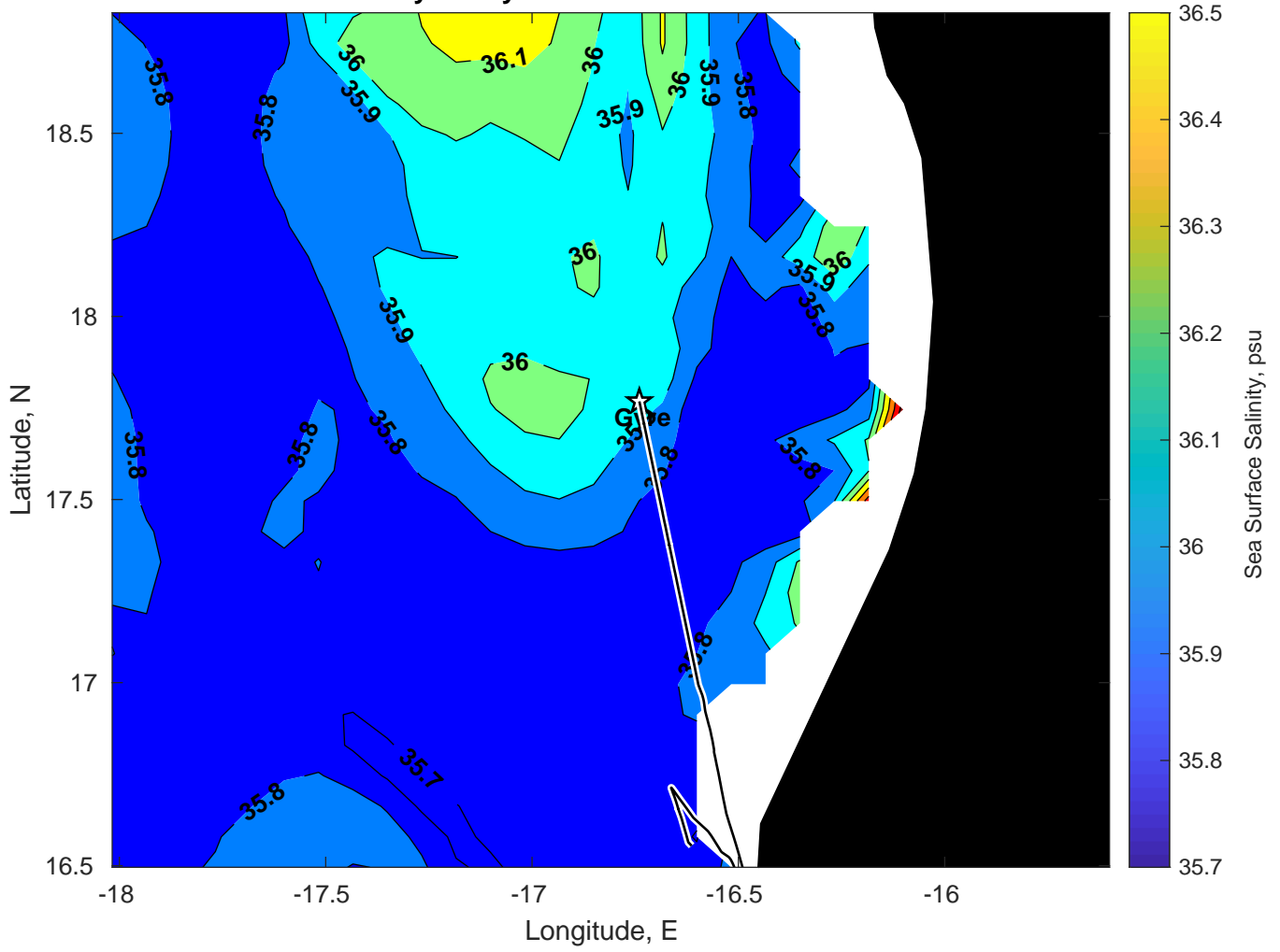
Surface Salinity for Gyre at 18-Mar-2025 00:00:00
