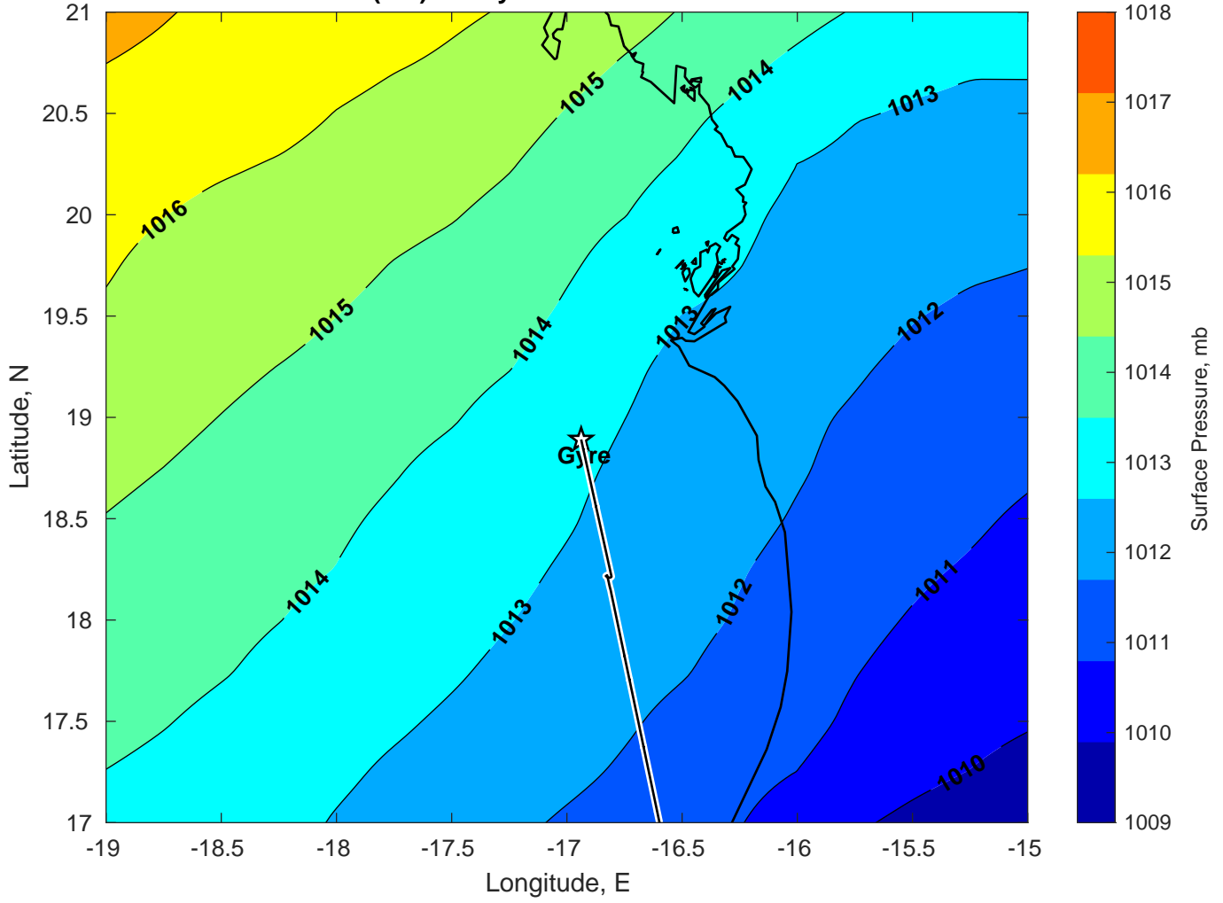
Surface Pressure (mb) for Gyre at 19-Mar-2025 00:00:00
